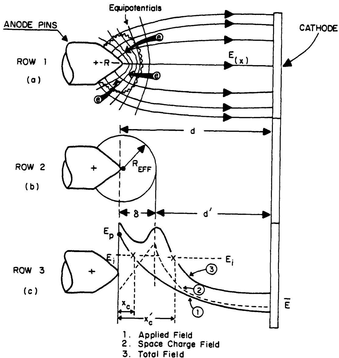
Figure 5. (a) Schematic of Field Lines and Equipotentials. (b) Apparent Dimensional Changes Due to Space Charge. (c) Applied, Space Charge and Total Field Distributions.
