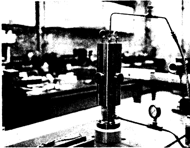
FIGURE 2. Photograph of Combustion Bomb
