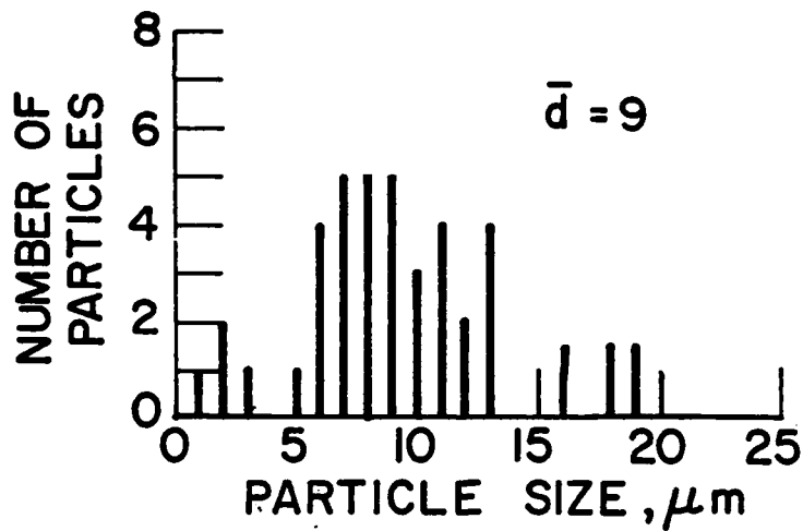
FIGURE 36. Particle Size Distribution (1615100580, NWC-2, P_c = 1000 psi)
