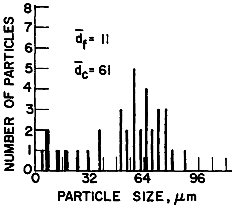
FIGURE 28. Particle Size Distribution (1600170480, WGS-6A, P_c = 1000 psi)
