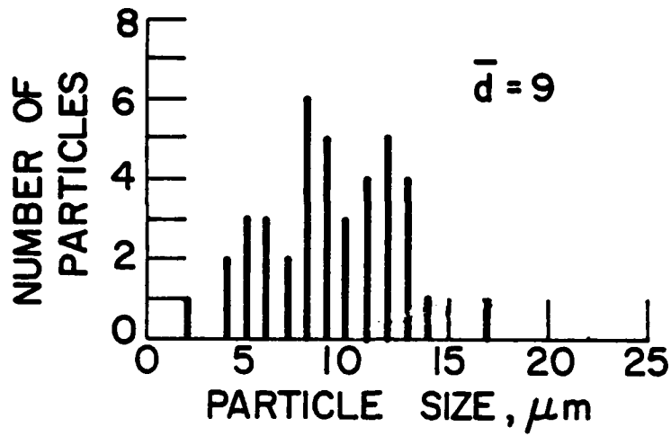
FIGURE 33. Particle Size Distribution (1230110580, NWC-1, P_c = 500 psi)
