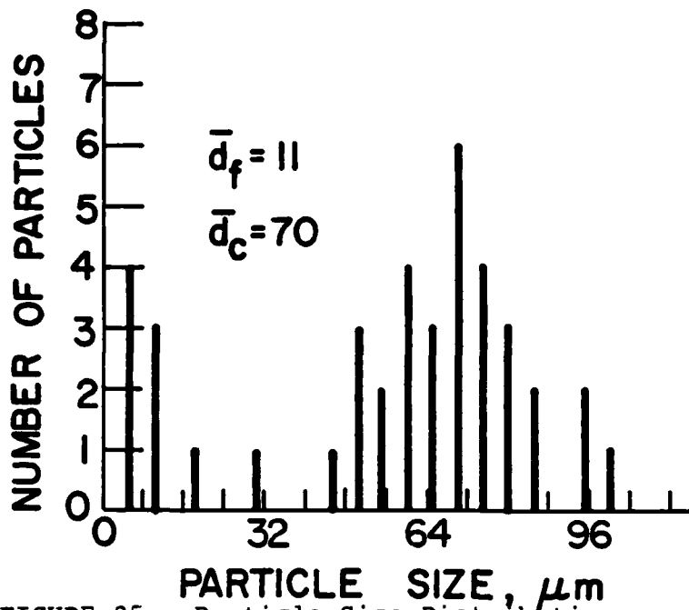
FIGURE 25. Particle Size Distribution (1445240480, WGS-5A, P_c = 500 psi)
