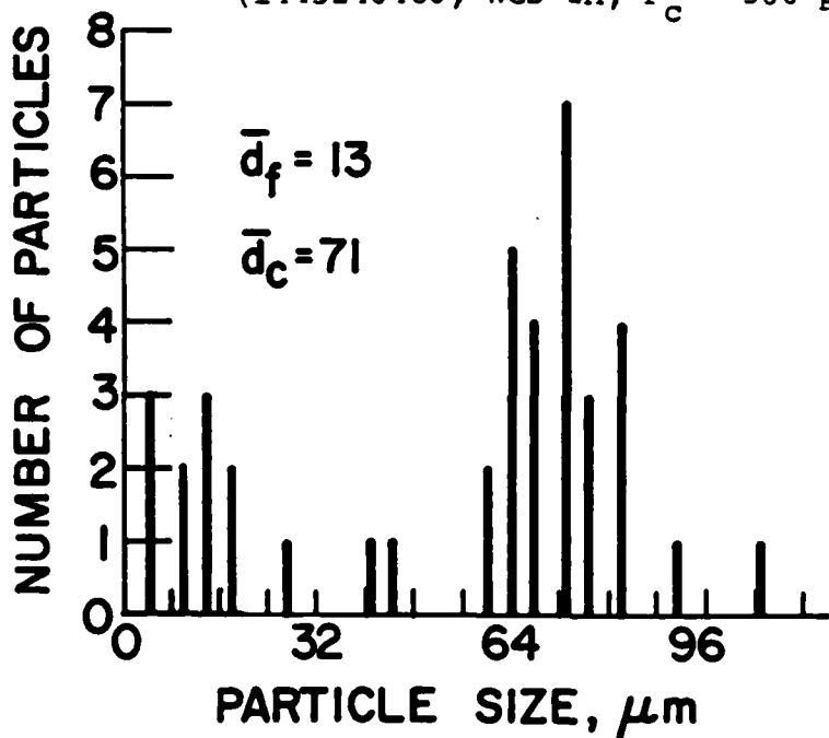
FIGURE 26. Particle Size Distribution (1445180480, WGS-5A, P_c = 1000 psi)
