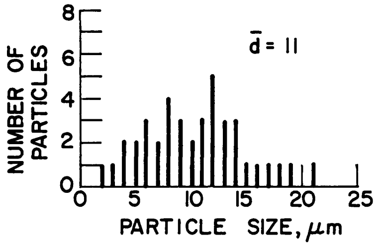
FIGURE 35. Particle Size Distribution (1200110580, NWC-2, P_c = 500 psi)
