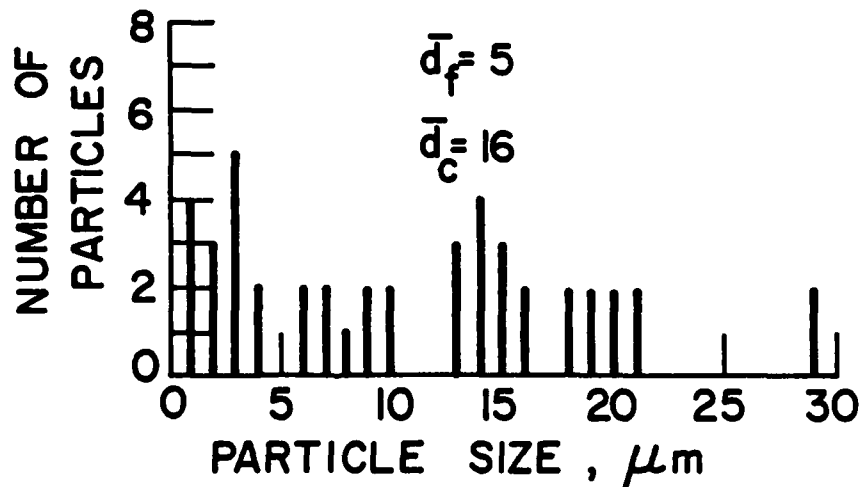
FIGURE 30. Particle Size Distribution (1400240480, WGS-7A, P_c = 1000 psi)
