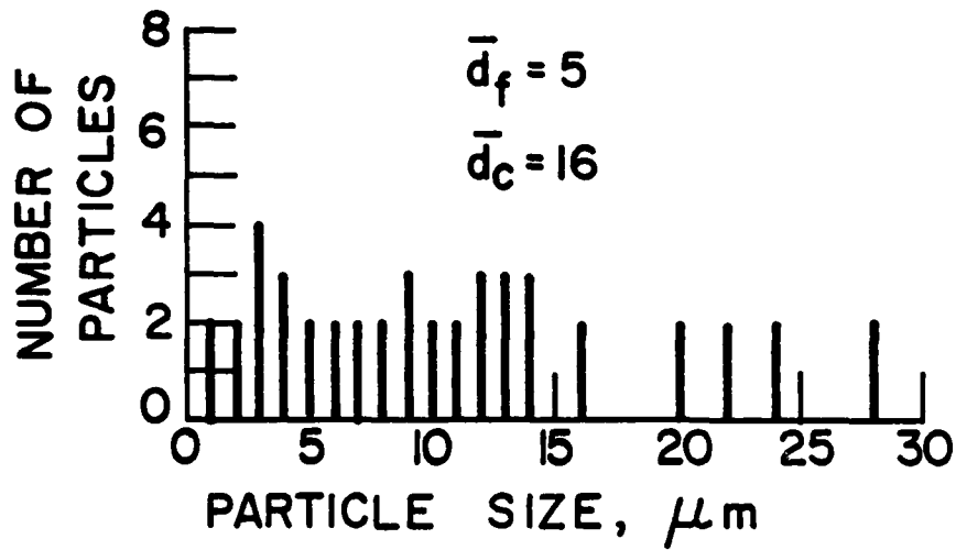
FIGURE 29. Particle Size Distribution (1215030580, WGS-7A, P_c = 500 psi)
