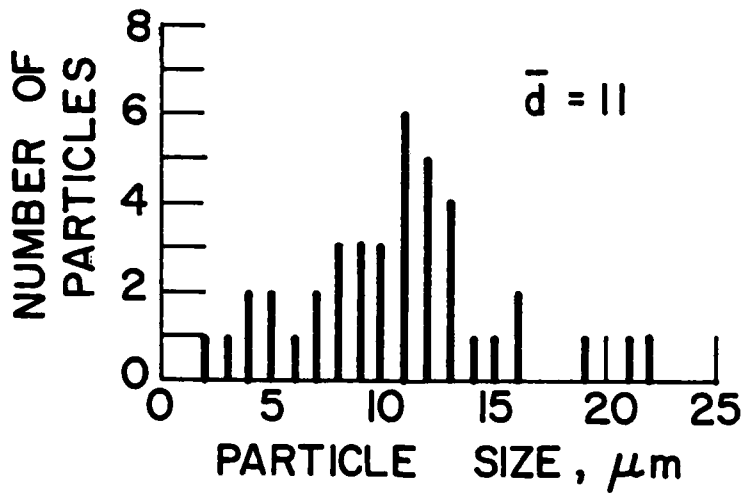
FIGURE 34. Particle Size Distribution (1500100580, NWC-1, P_c = 1000 psi)
