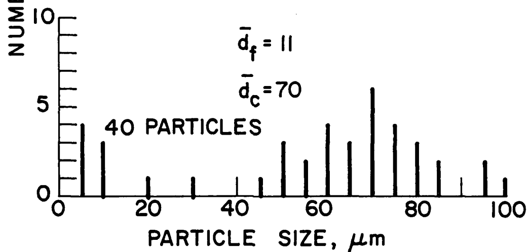
FIGURE 37. Comparison of 40 and 220 Particle Sample Distributions (14452400480, WGS-5A, P_c = 500 psi)
