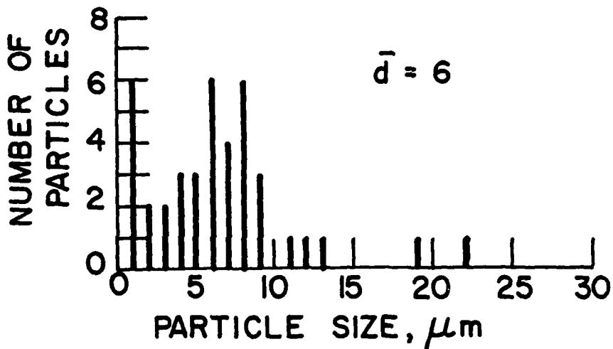
FIGURE 32. Particle Size Distribution (1500210480, WGS-7, P_c = 1000 psi)
