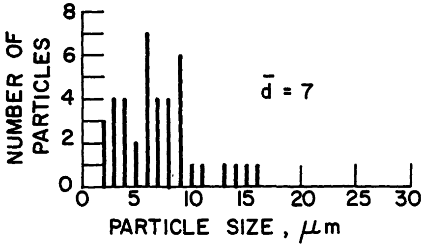
FIGURE 31. Particle Size Distribution (1100030580, WGS-7, P_c = 500 psi)
