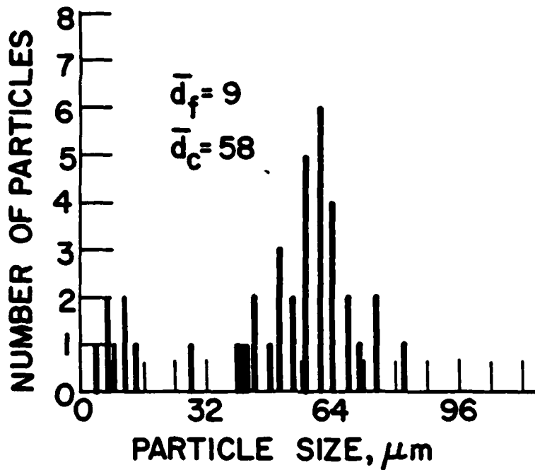
FIGURE 27. Particle Size Distribution (1030030580, WGS-6A, P_c = 500 psi)
