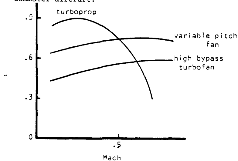
Variable Pitch Fan, Turboprop, and Turbofan Efficiencies.
