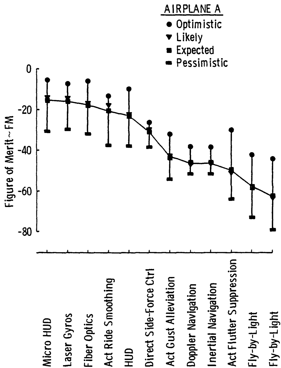
Fig. B.3. Airplane A PLOE Figure of Merit Comparisons (concluded)
