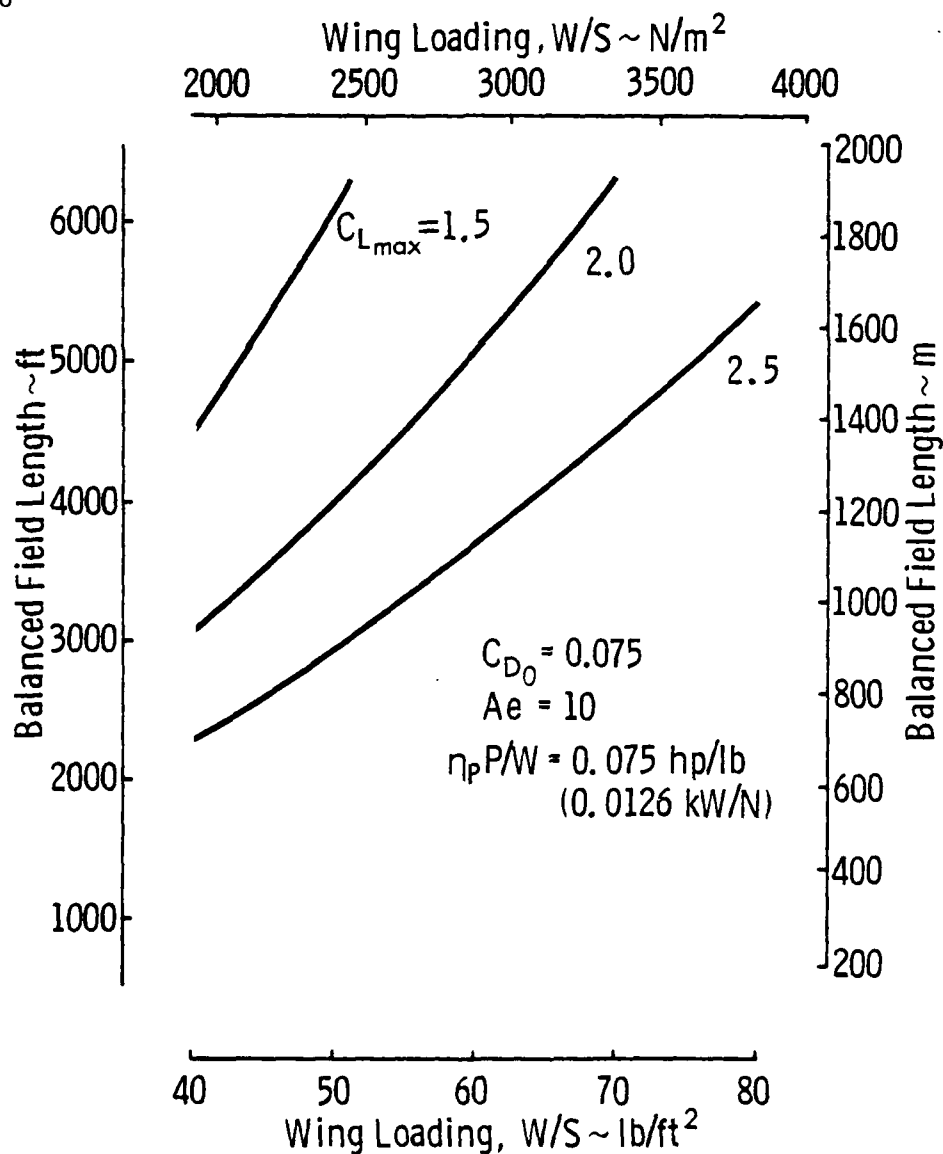
Fig. 5.6. Commuter Balanced Field Length Studies
