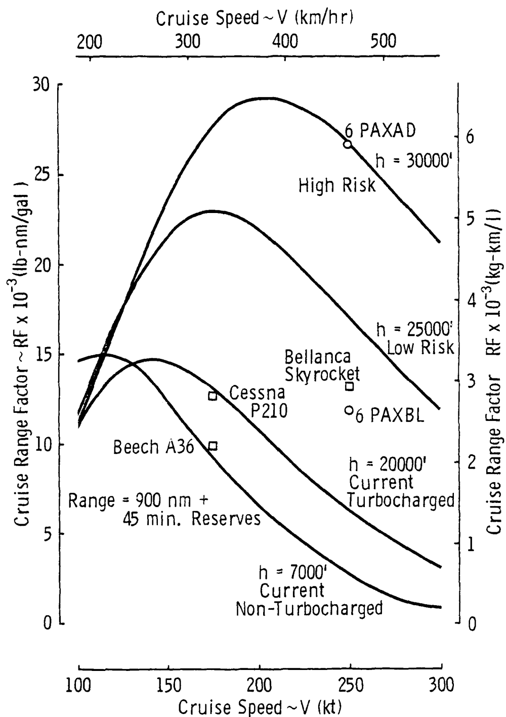
Fig. 5.19. 6-Passenger Range Factor Comparisons
