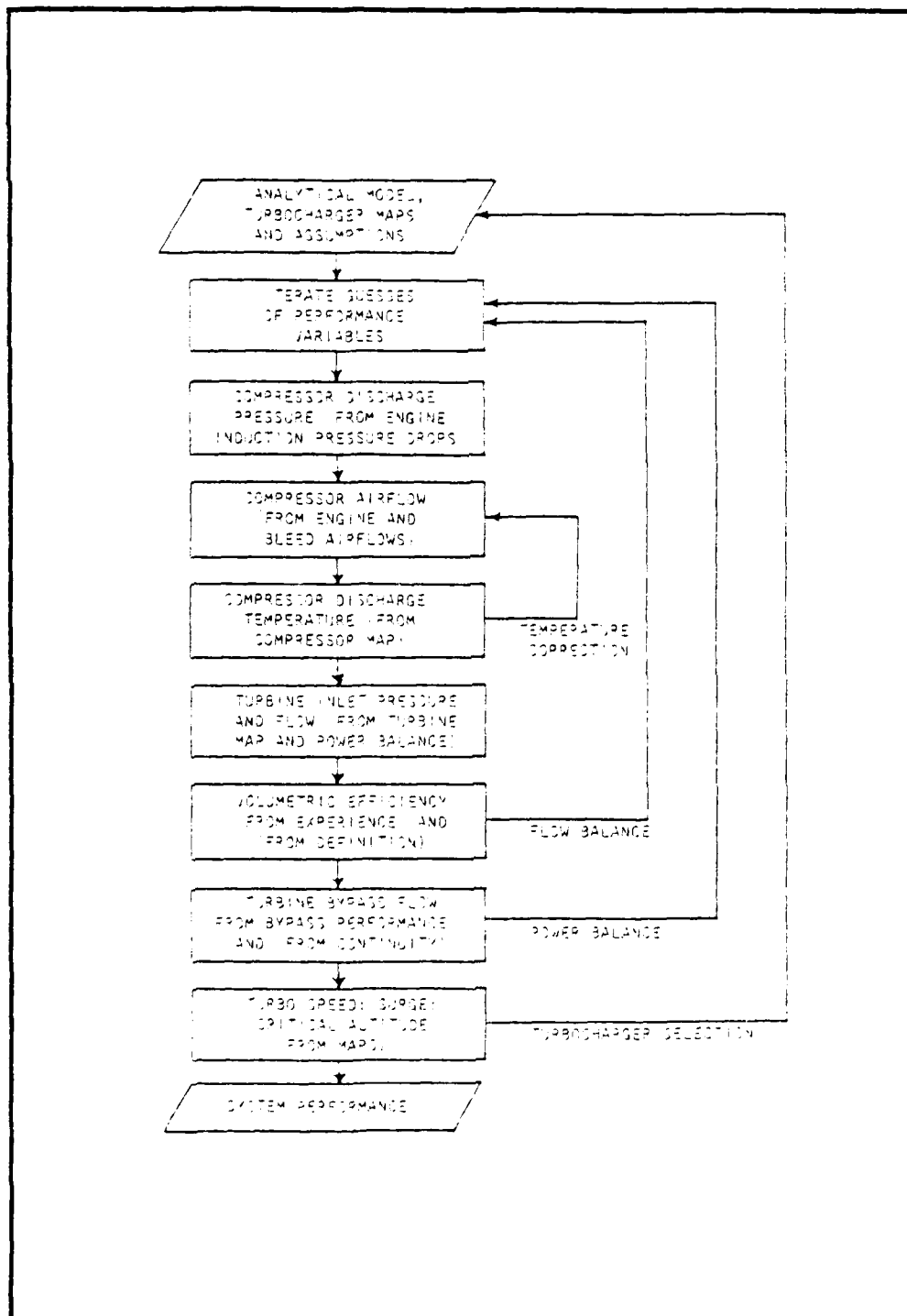
Turbocharger Design Logic
