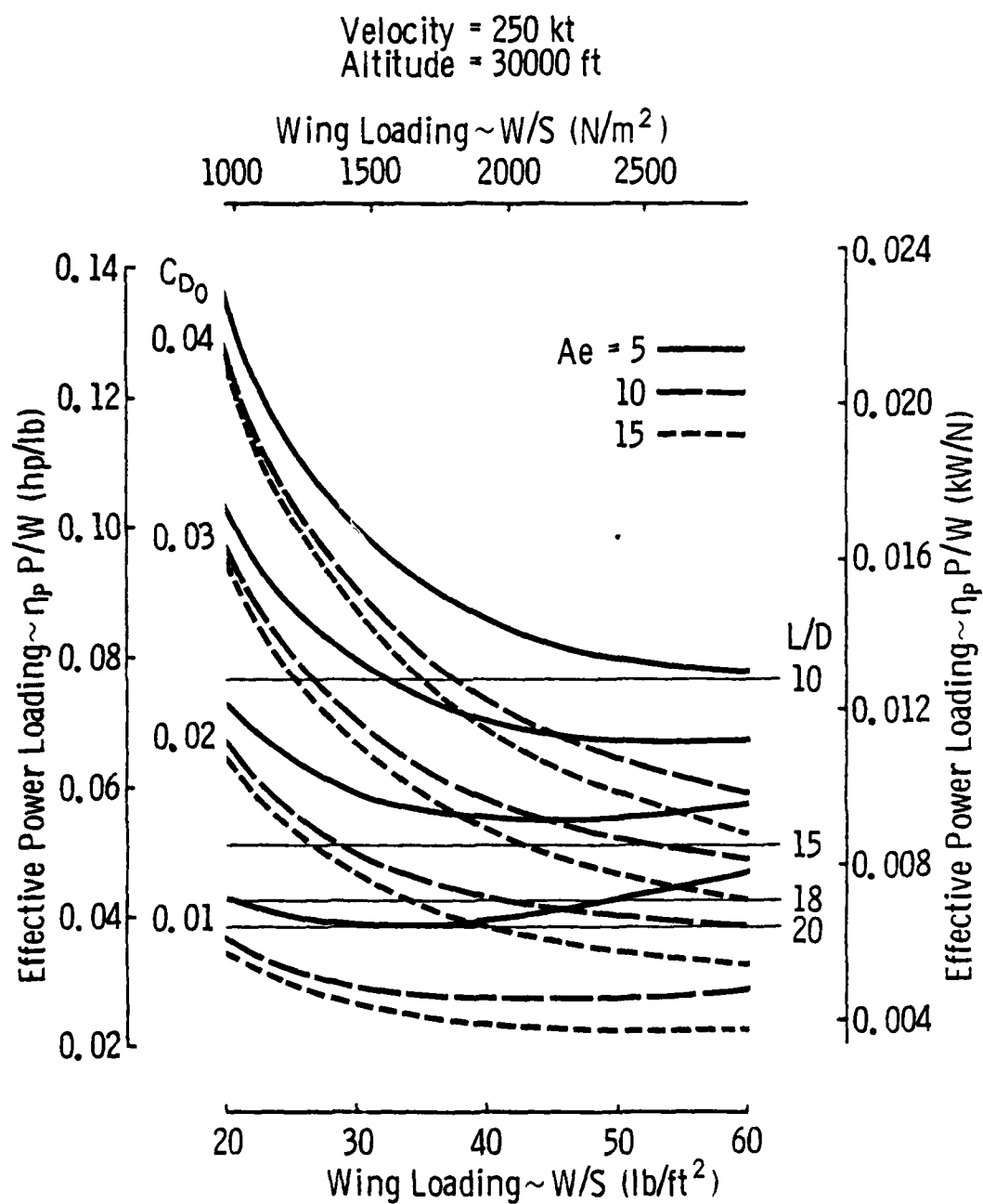
Fig. 5.2. 6-Passenger Cruise Trade Studies (at 30000 ft)
