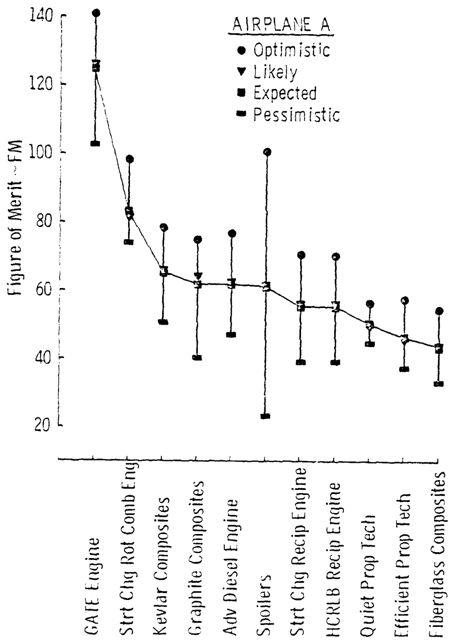
Fig. 8.3. Airplane A PLAE Figure of Merit Comparisons
