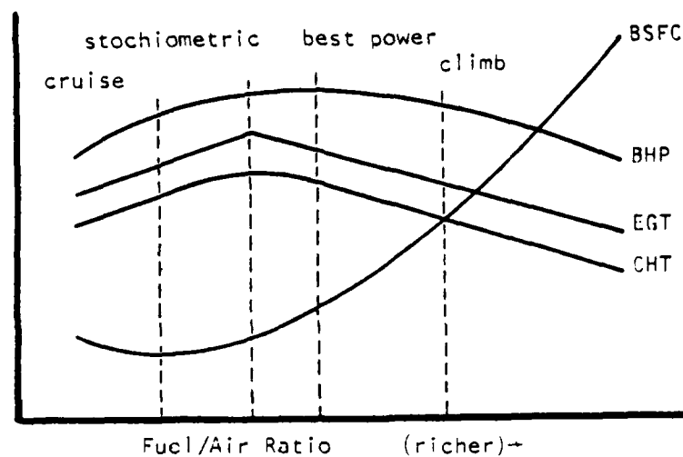
Engine Operating Characteristics
