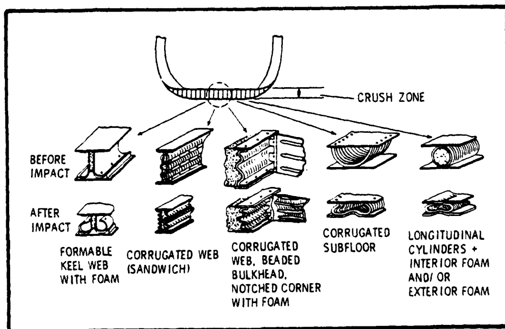
Fig. 4.12. Energy Absorbing Floor Concepts.
