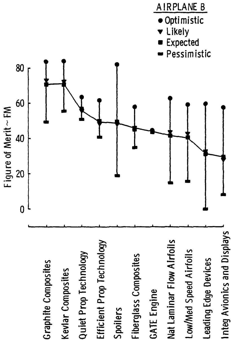
Fig. B.4. Airplane B PLOE Figure of Merit Comparisons
