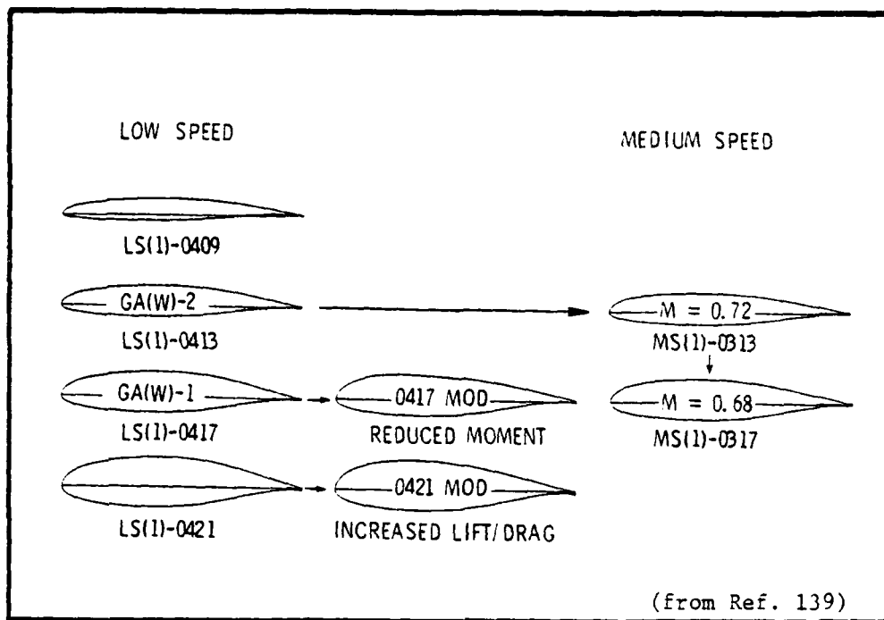
Fig. 4.5. Design Family of NASA Low-Speed Airfoils.
