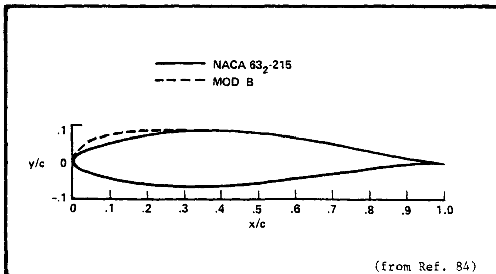
Fig. 4.6. Modification to NACA 63 2 -215 Airfoil.
