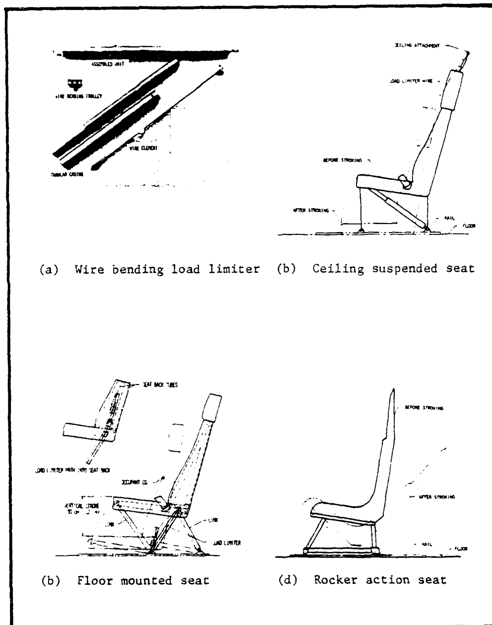
Fig. 4.11. Load Limiting Seat Concepts.
