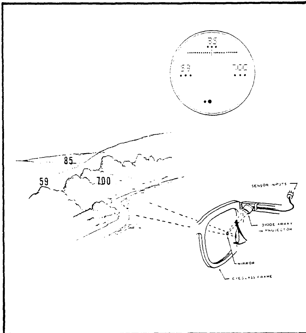
Fig. 4.20. Micro HUD Image Display.
