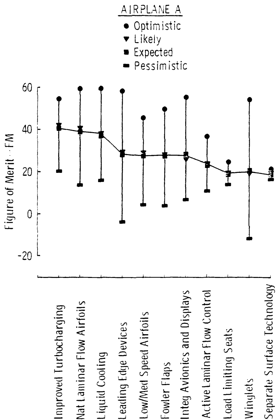
Fig. 3.5. Airplane A PLDE Figure of Merit Comparisons (continued)
