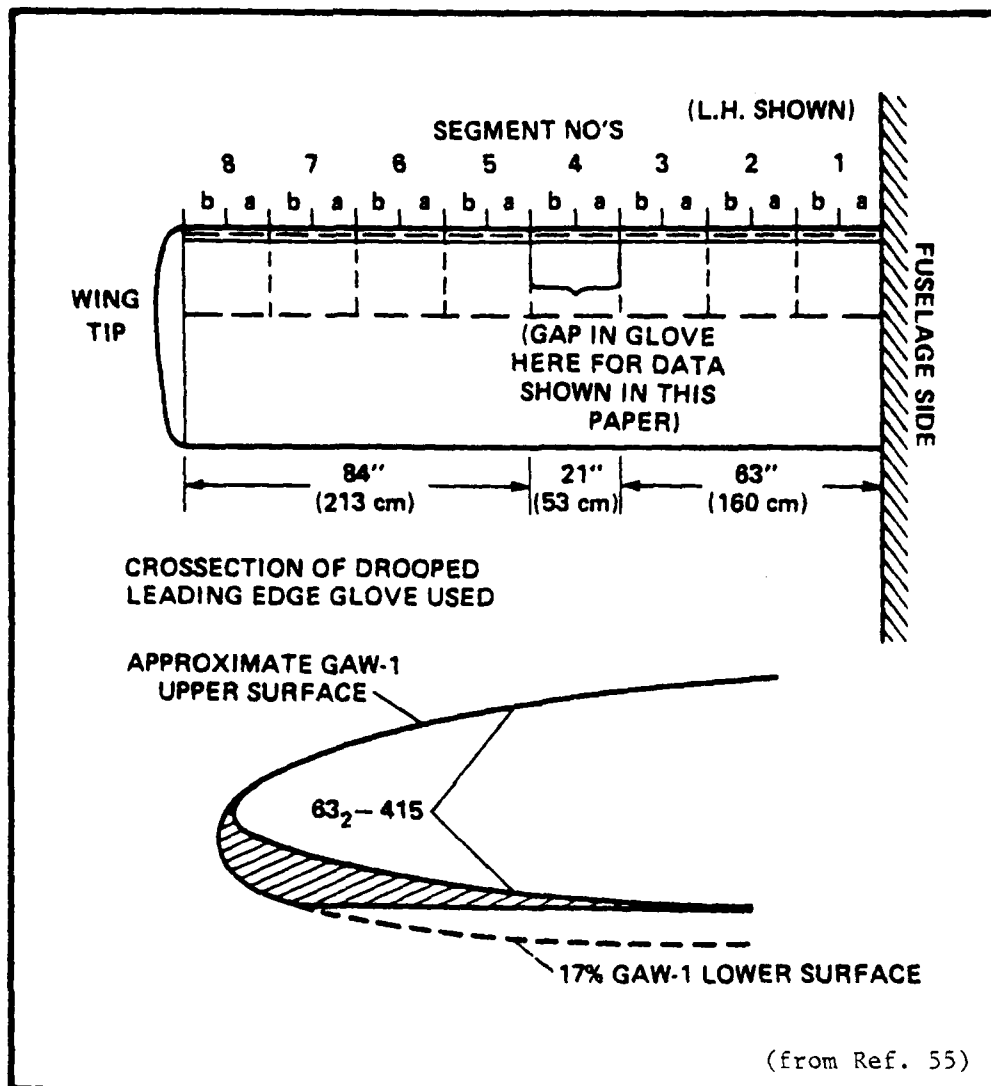
Fig. 4.9. Leading Edge Modification for Stall/Spin Alleviation
