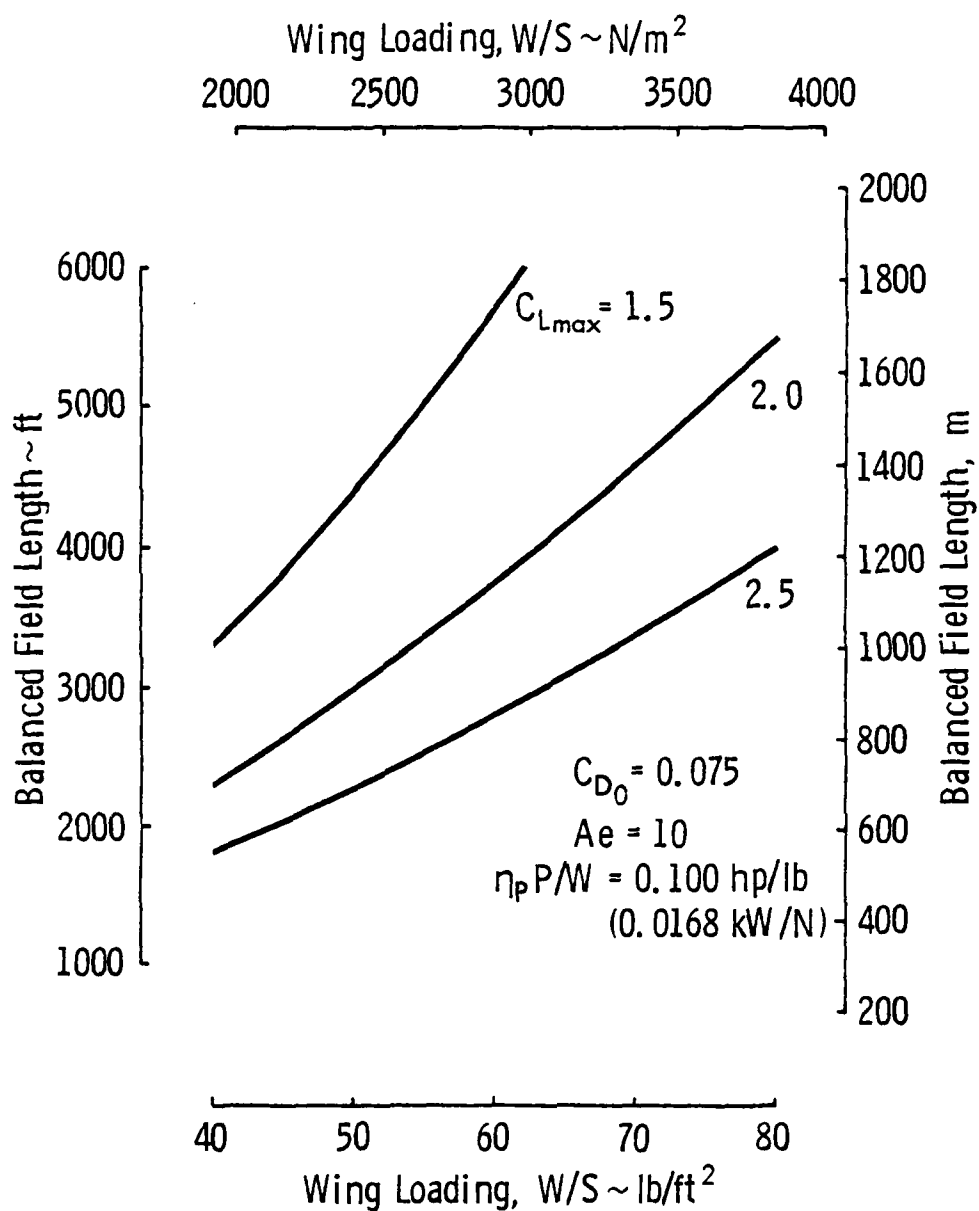
Fig. 5.7. Commuter Balanced Field Length Studies
