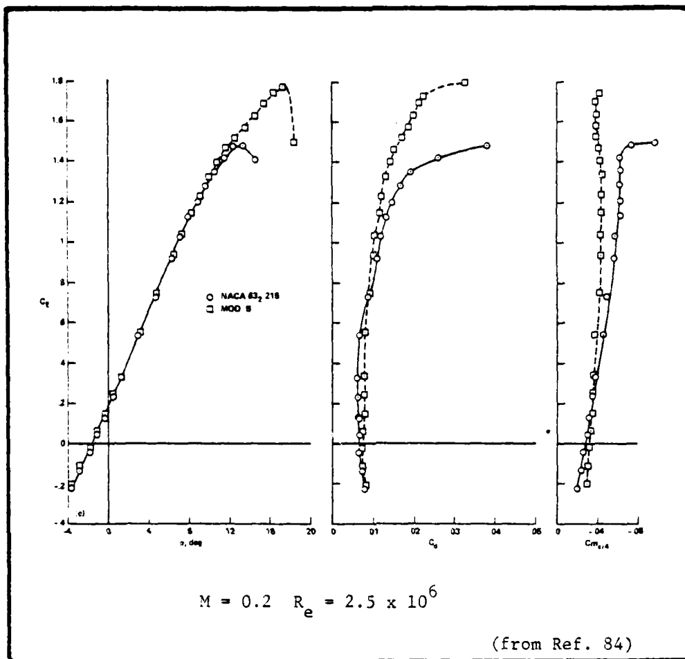
Fig. 4.7. Experimental Results of a Modification to an NACA 63 2 -215 Airfoil.
