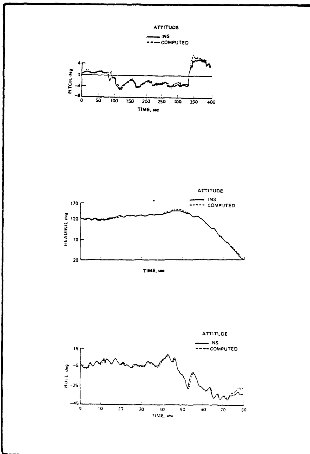
Fig. 4.21. Comparison of Pitch, Heading, and Roll Computations.
