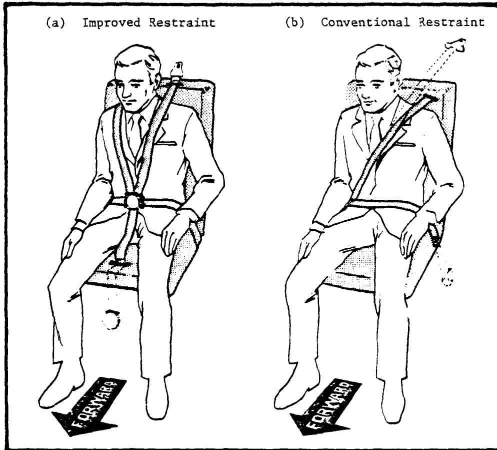
Fig. 4.13. Five Point Improved Restraint vs Conventional Restraint
