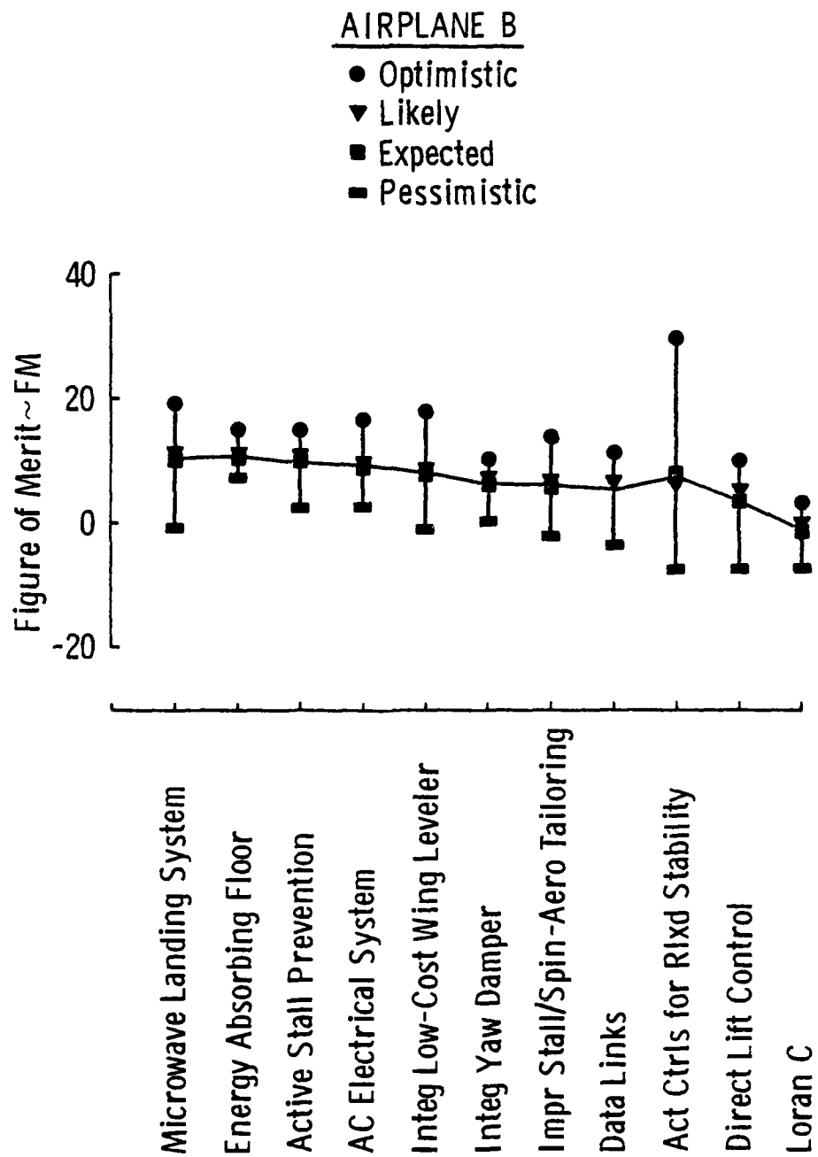
Fig. B.4. Airplane B PLOE Figure of Merit Comparisons (continued)
