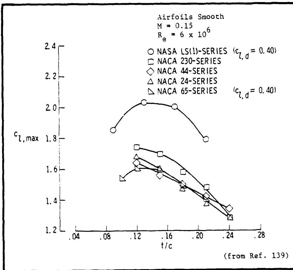
Fig. 4.3. c_{l,max} vs t/c of NASA Low-Speed and NACA Airfoils.
