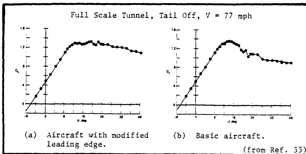
Fig. 4.10. Flat-Topped Lift Curve from Leading Edge Modification for Stall/Spin Alleviation.
