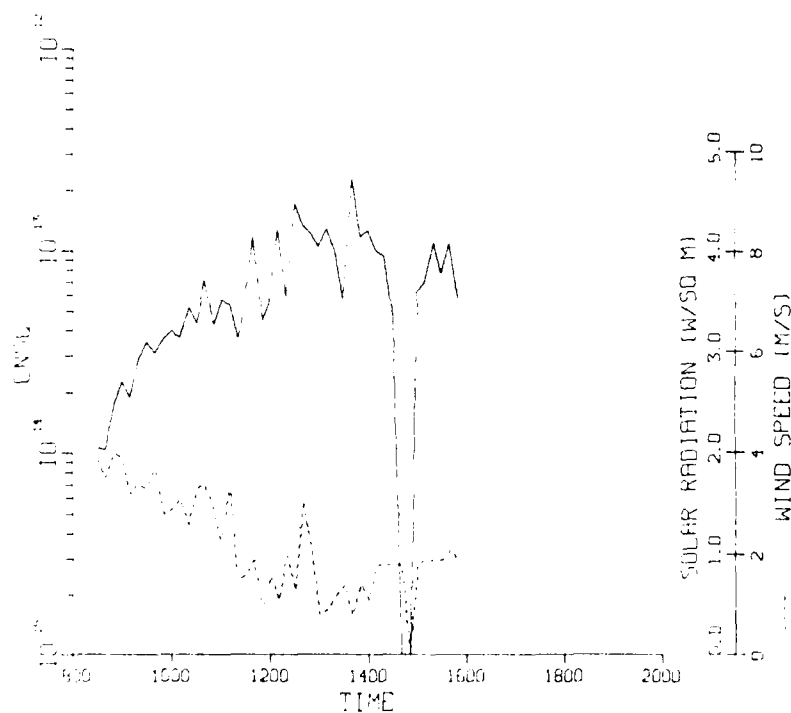
Fig. A-4 - Solar radiation, windspeed, and C_2 at the optical transmitter meteorological station on 11 August 1978
