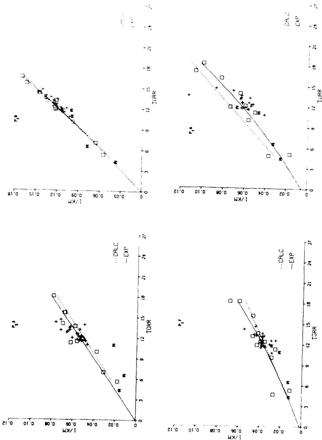
Fig. 2 — Measured D 2 O molecular absorption coefficient dependence on water vapor partial pressure. — Cape Canaveral Air Force Station, Fla.; +, TRW Capistrano Test Site Calif.; W, WSMR N. Mex.; — least squares fit to Florida data; —, SAI algorithm [1].
