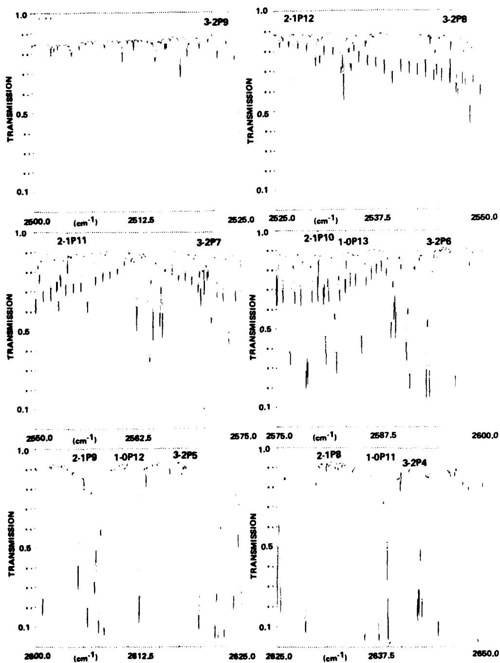
Fig. 18 - HITRAN predictions for atmospheric transmission over 6.4-km path with midlatitude summer conditions scaled to 1133 Pa (8.8 torr) H_2O , 33°C air temperature, and 88 \times 10^3 Pa (660 torr) total pressure
