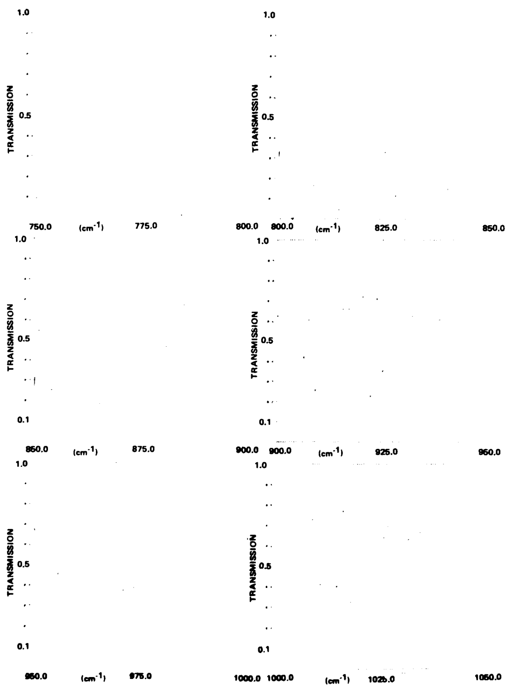
Fig. 29 — HITRAN predictions for atmospheric transmission over 6.4 km path with midlatitude summer conditions scaled to 1067 Pa (8.0 torr) \text{H}_2\text{O} at 31°C temperature with a 1.4 \text{ cm}^{-1} (sm ^{-1} ) instrument function convolution
