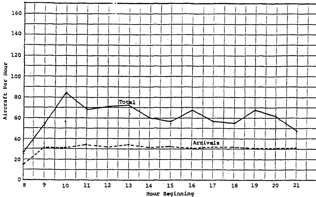
FIGURE 3A--AVERAGE RUNWAY FLOW RATES
