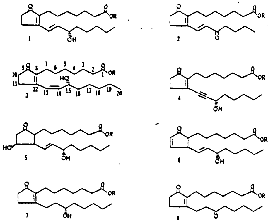
Chemical structures of prostaglandins referred to in text: (1) PGB 1 , (2) 15-dehydro-PGB 1 , (3) cis -PGB 1 , (4) 13, 14-dehydro-PGB 1 , (5) PGE 1 , (6) PGA 1 , (7) 13, 14-dehydro-PGB 1 , and (8) 13,14-dihydro-15-dehydro-PGB 1 . The conventional numbering system for prostaglandins referred to in the text is illustrated in the example of cis -PGB 1 (3).
