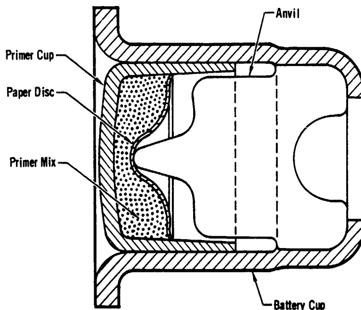
Figure 2 Shotshell or Battery Cup Primer
