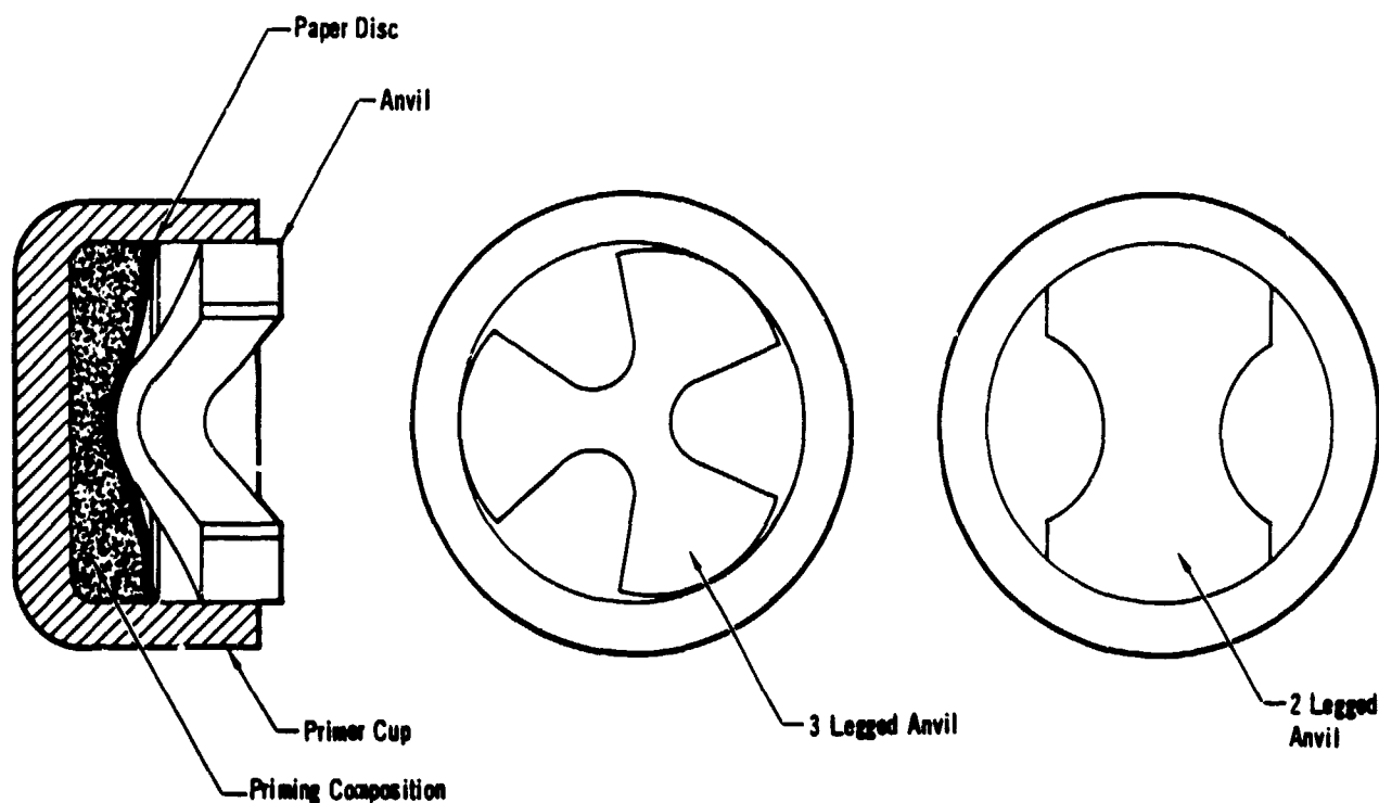
Figure 1 Commercial or Military Center Fire Primer
