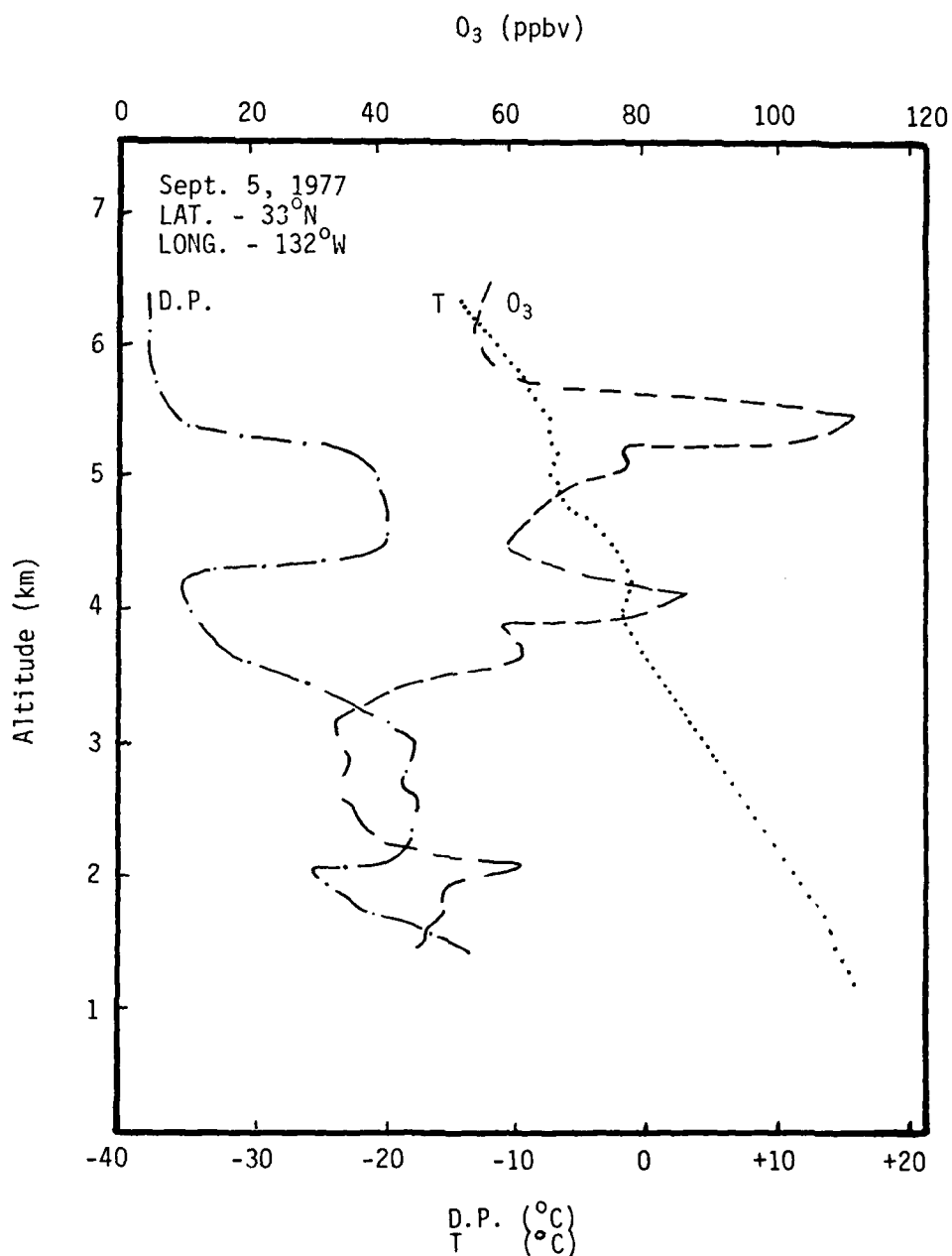
Figure 46. Representative Vertical Profile of Ozone, Dew-point, and Temperature as Measured by Project GAMETAG.
