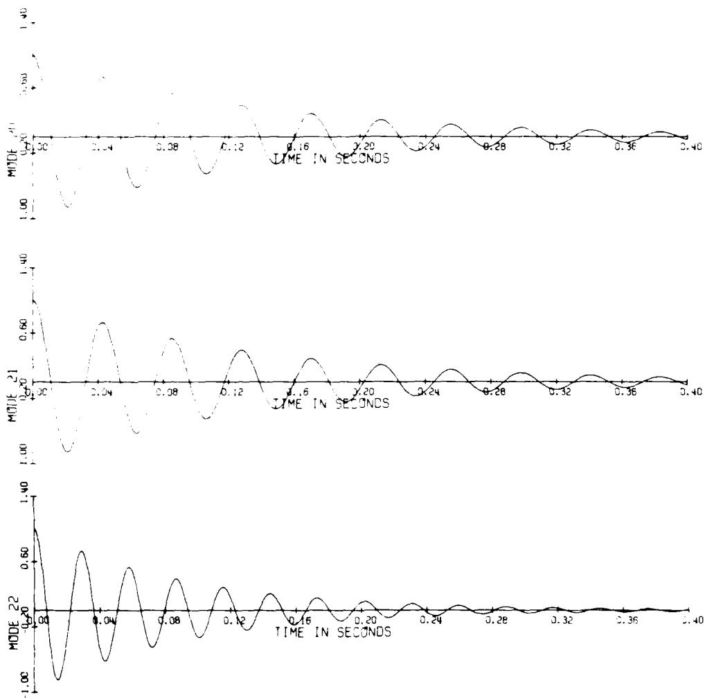
Figure 19. Open-loop feedback response (sheet 3 of 3).
