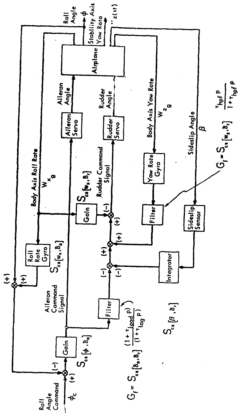
Figure A-5. Functional block diagram of the lateral-directional flight control system.
