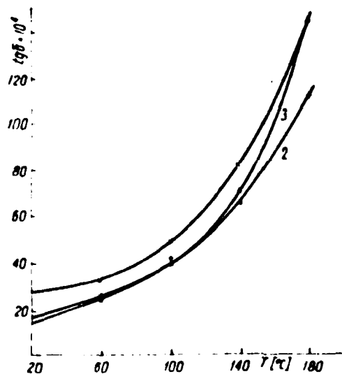
Fig. 11. Temperature of dependence of tg of angle of loss of insulating layers
