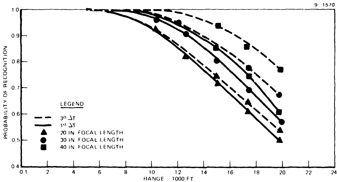
FIGURE 16 RESULTS OF MODELING SENSOR FOCAL LENGTH
