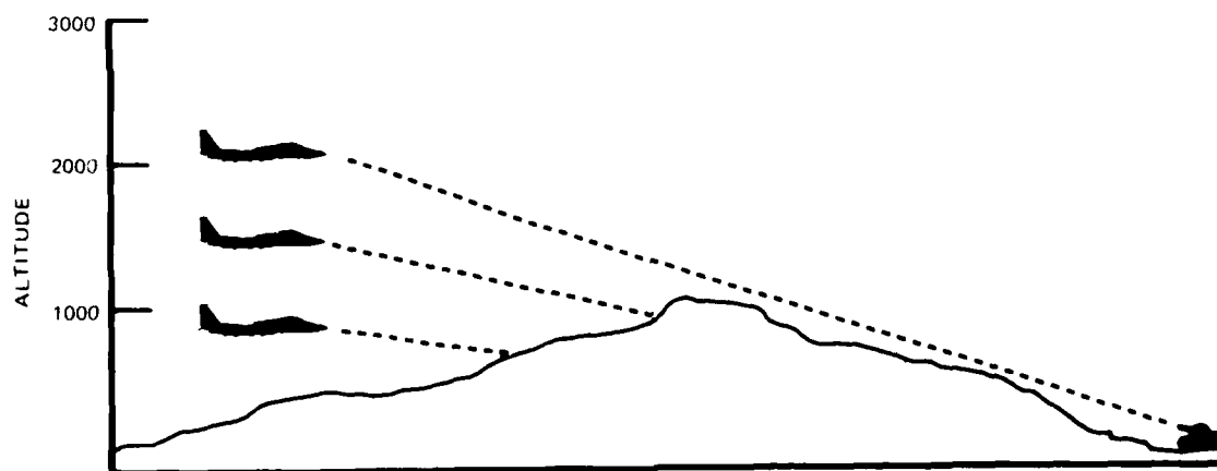
FIGURE 9 TERRAIN MASKING AS A FUNCTION OF ALTITUDE
