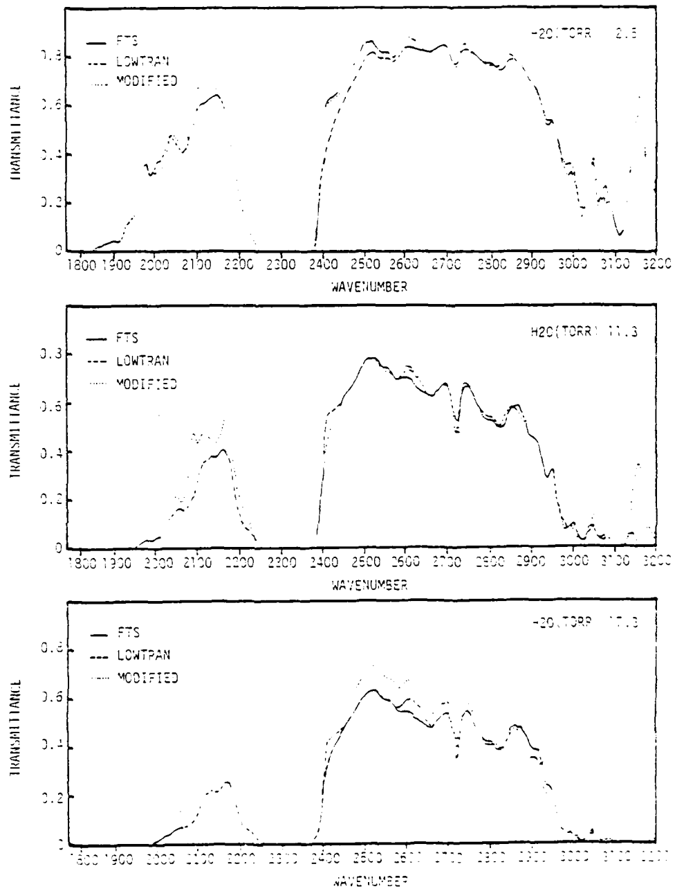
Figure 2. Comparison of NPL Fourier Transform Spectrometer (FTS) for a 5 km path with LOWTRAN Predictions. Note discrepancy between 2000 and 2250 \text{cm}^{-1} (4.0 - 4.4 \mu\text{m} ).
