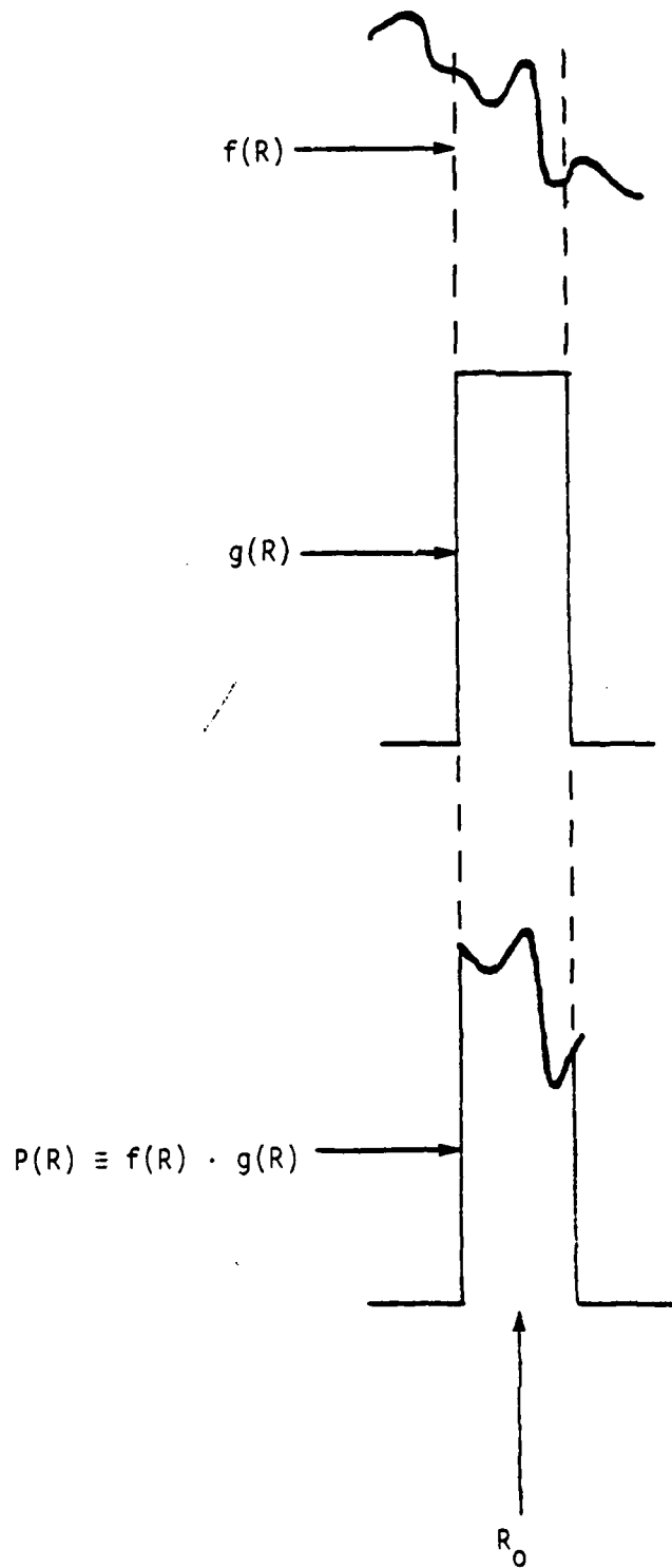
Figure 1. Action of Ideal Size-Binning Filter in Developing Particulate Output Count per Size Bin.
