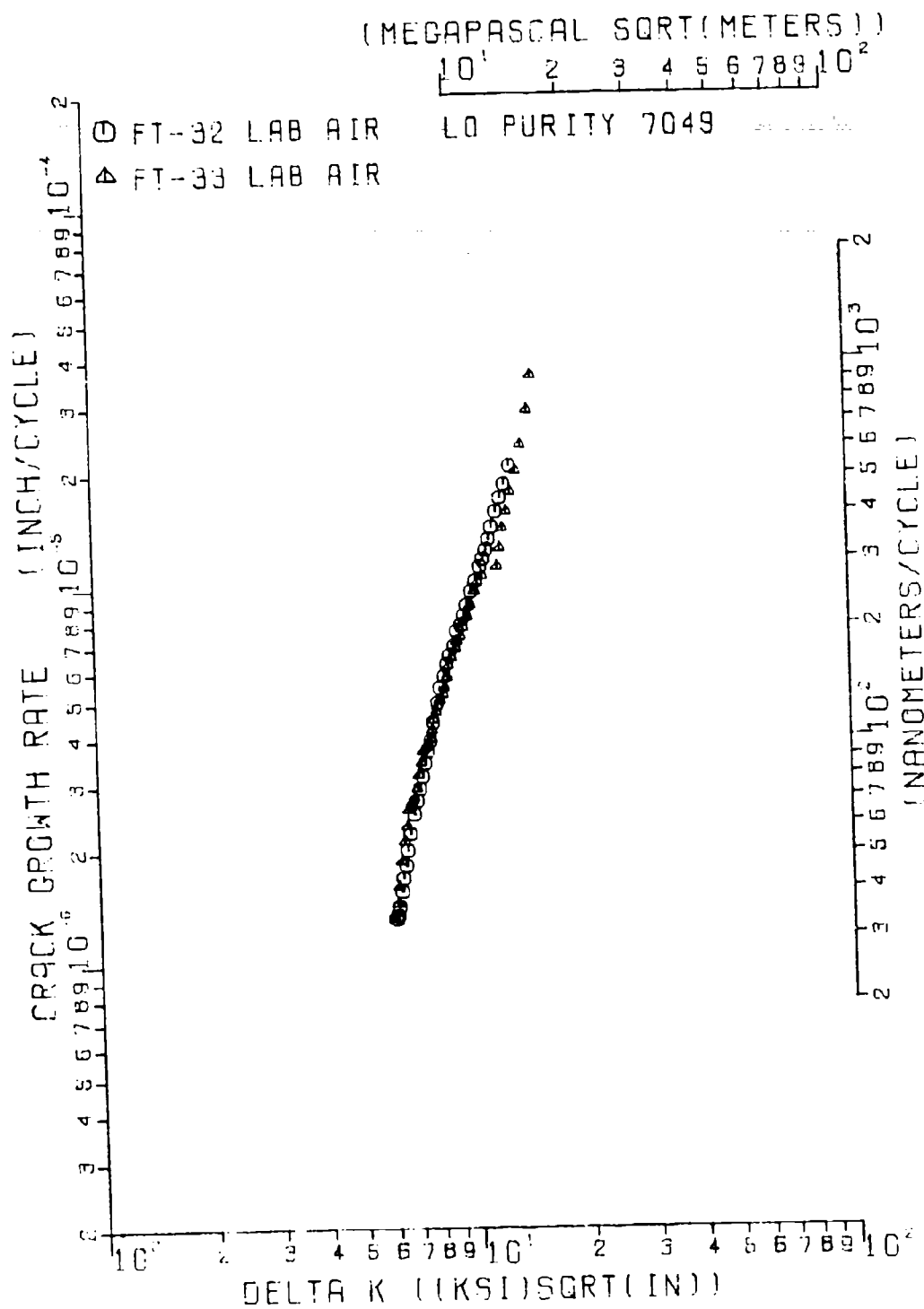
Figure 22. FCGR Data for Low Purity 7049; R = 0.1, Freq. = 30Hz, T-L Orientation
