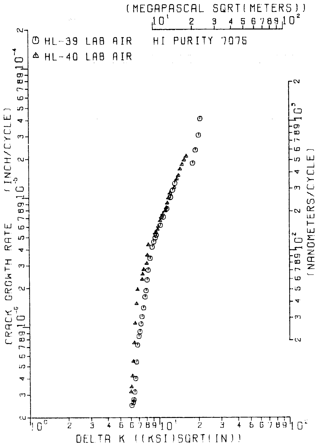
Figure 16. FCGR Data for High Purity 7075; R = 0.1, Freq. = 30Hz, L-T Orientation
