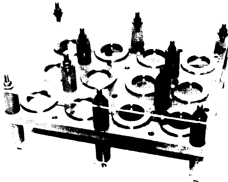
Figure 3. Fully assembled test fixture A (above), and the assembled test fixture with the front plate removed, prior to immersion (below).
