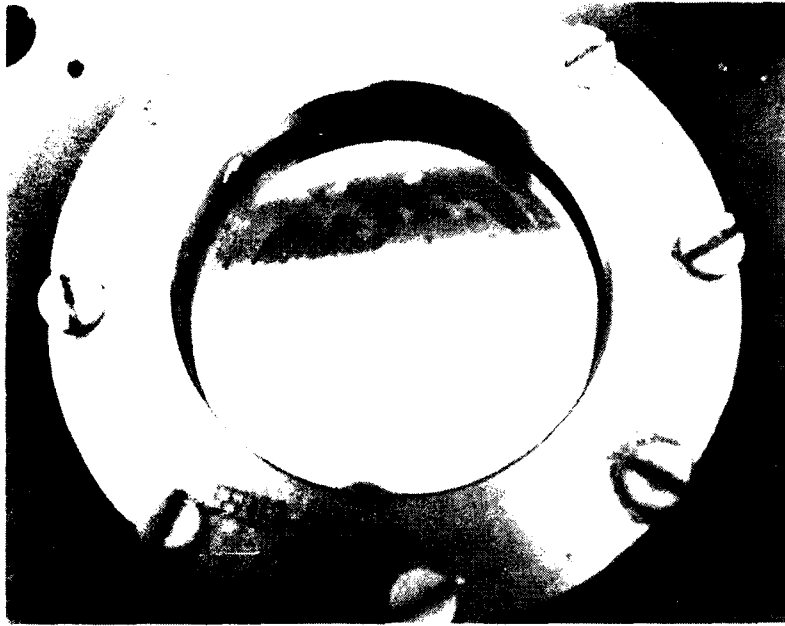
Figure 13. A germanium specimen with the Optic Electronic XF129 AR coating, after 4 months in San Diego Bay.
