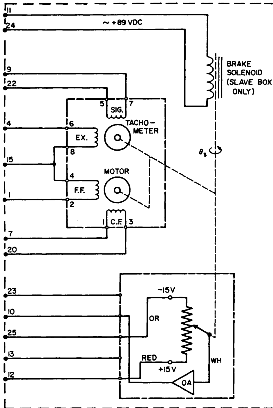
Fig. B.5. Gearbox Schematic (from Brooks[3])
