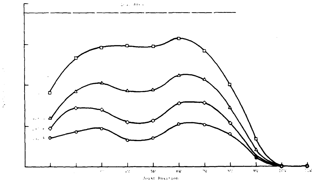
Figure A.14 Deflection versus Joist Position for Indicated Load Levels - West Side, Second Load Test
