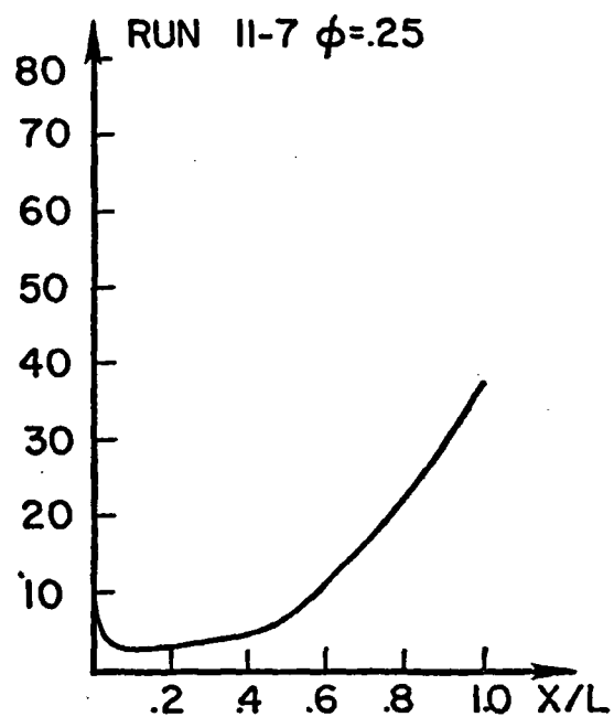
FIGURE 22c. THE \frac{i_{chem}}{R^2/D_0} vs X/L FOR DIFFERENT \phi
