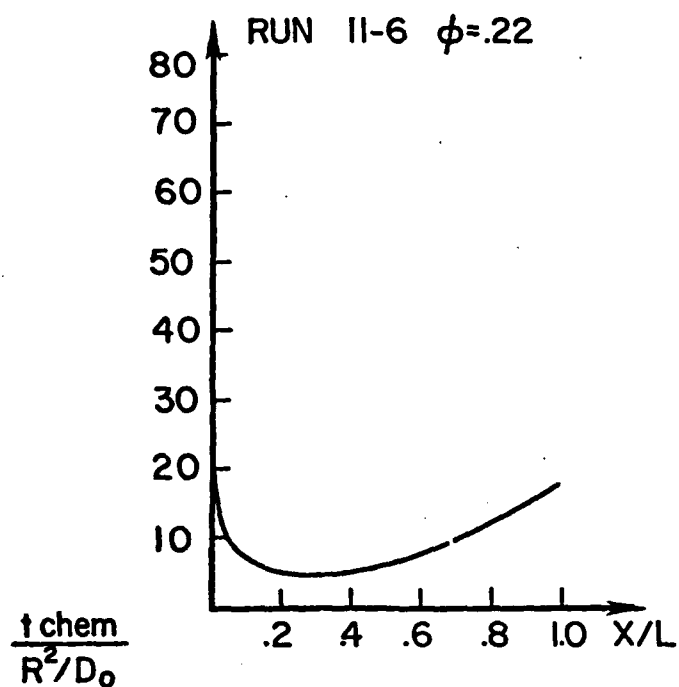
FIGURE 22c. THE \frac{i_{chem}}{R^2/D_0} vs X/L FOR DIFFERENT \phi
