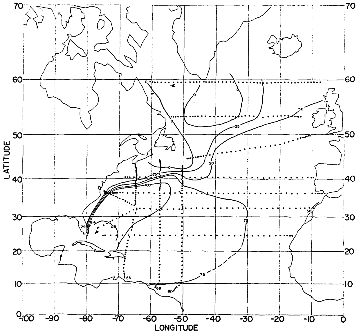
2. Sea surface, relative to geoid, computed from circulation in figure 1 (Wunsch, 1980).
