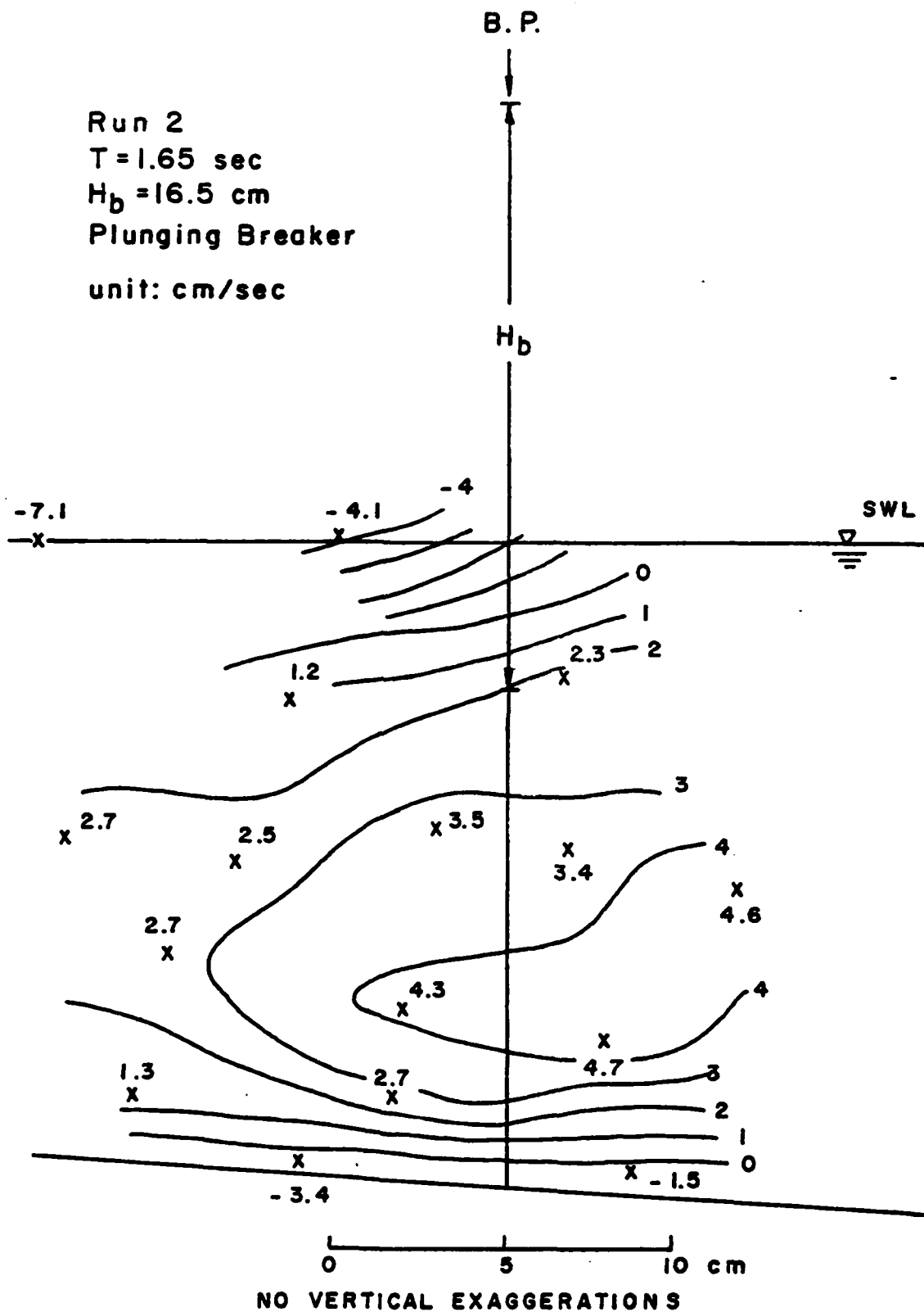
Fig. 6b. Drift-velocity distribution around the breaking point.
