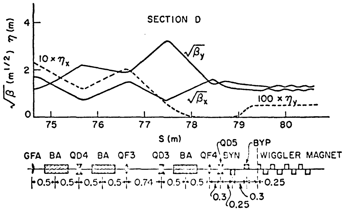
Figure 5b. Lattice Functions in Sections C and D.
