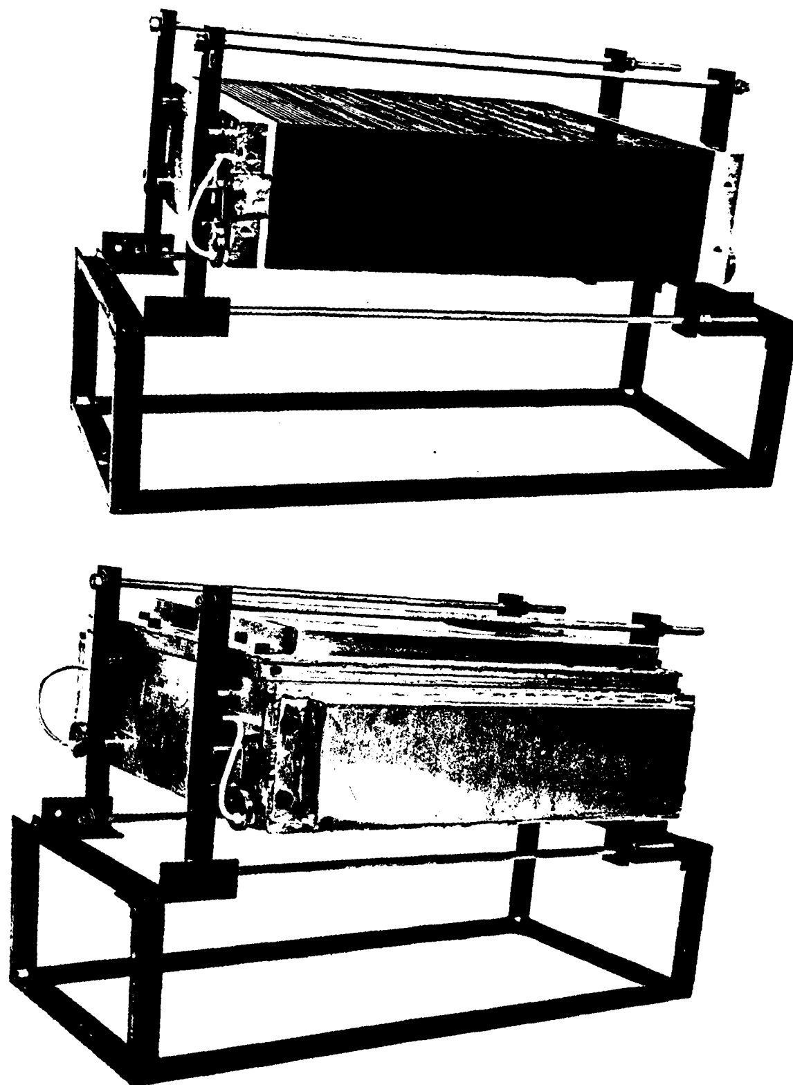
FIGURE 48 80-CELL STACK WITHOUT AND WITH GAS MANIFOLDS INSTALLED
