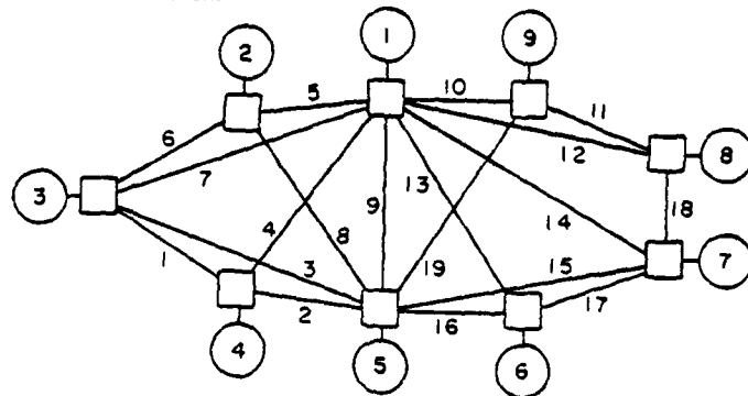
Figure 3-1. Interconnection Network
