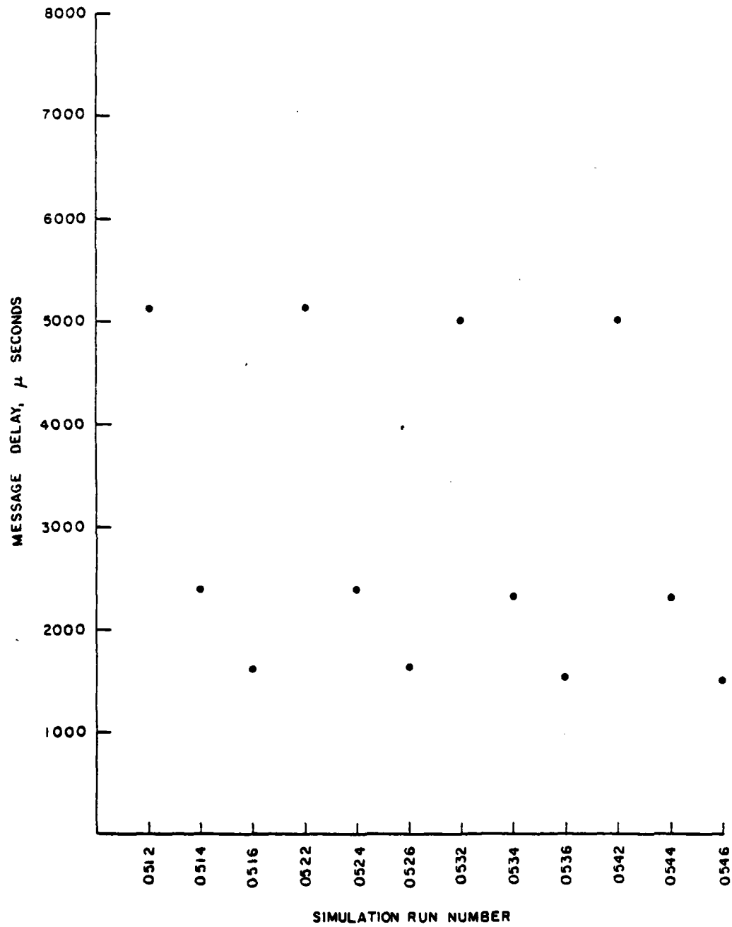
Figure D-1. Global Bus Network Simulation Overall Mean Message Delay, \mu Seconds Using RN1 Random Number Seed 05 Run Series
