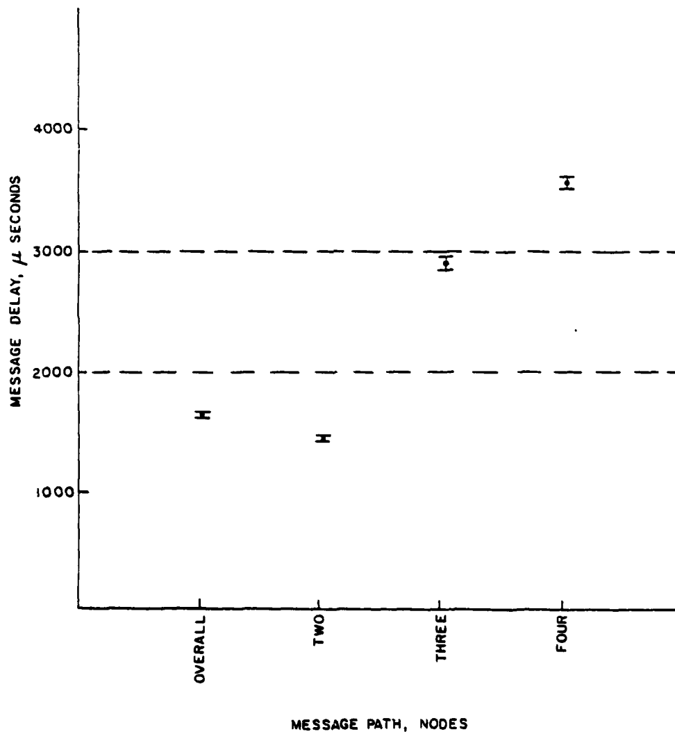
Figure 5-4. Global Bus Network Simulation Message Delay, \mu Seconds With 90% Confidence Interval - Run Number 1038
