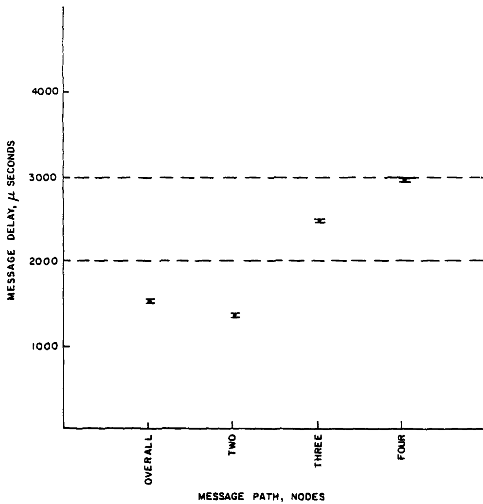
Figure 5-3. Global Bus Network Simulation Message Delay, \mu Seconds With 90% Confidence Interval - Run Number 0548
