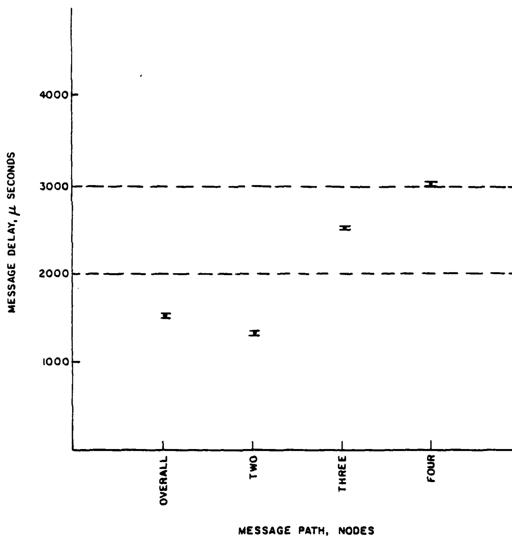
Figure 5-2. Global Bus Network Simulation Message Delay, \mu Seconds With 90% Confidence Interval - Run Number 0536
