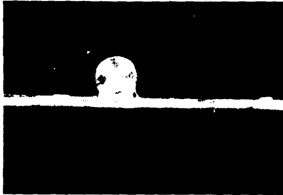
FIG. 4. Microsphere mounted on nylon filament. This microsphere is 85 \mu in diameter.
