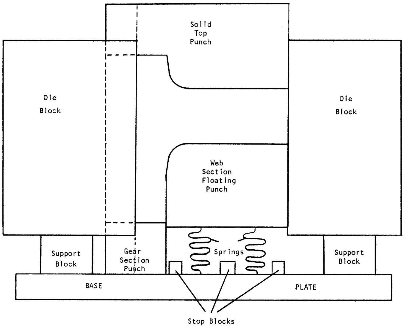
Figure 7. Split Punch Compaction Die Set Used to Compact the Six Outer Segments of the Preform.
