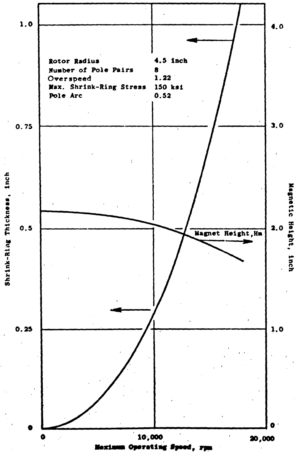
Figure 12. Shrink Ring Thickness and Magnet Height versus Maximum Operating Speed of a PM Rotor.
