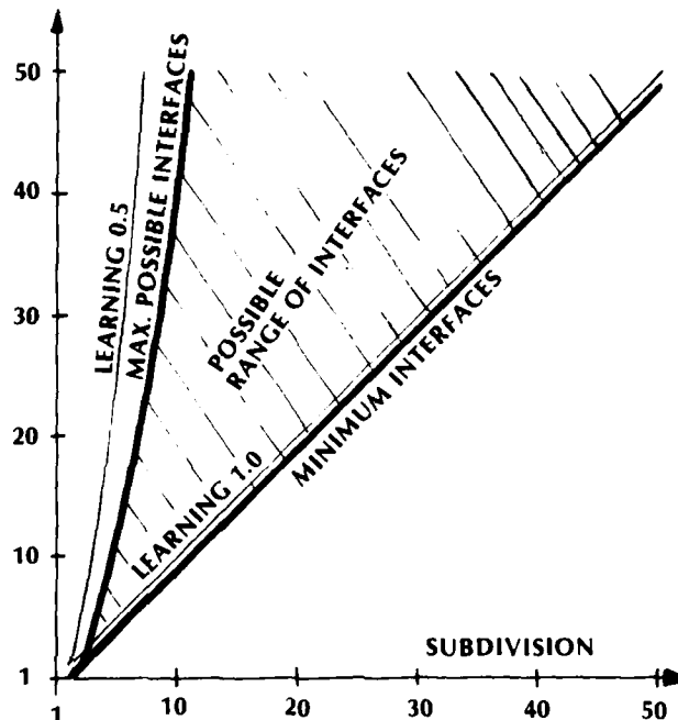
FIGURE 6B Range of Interfaces (Linear Form)
