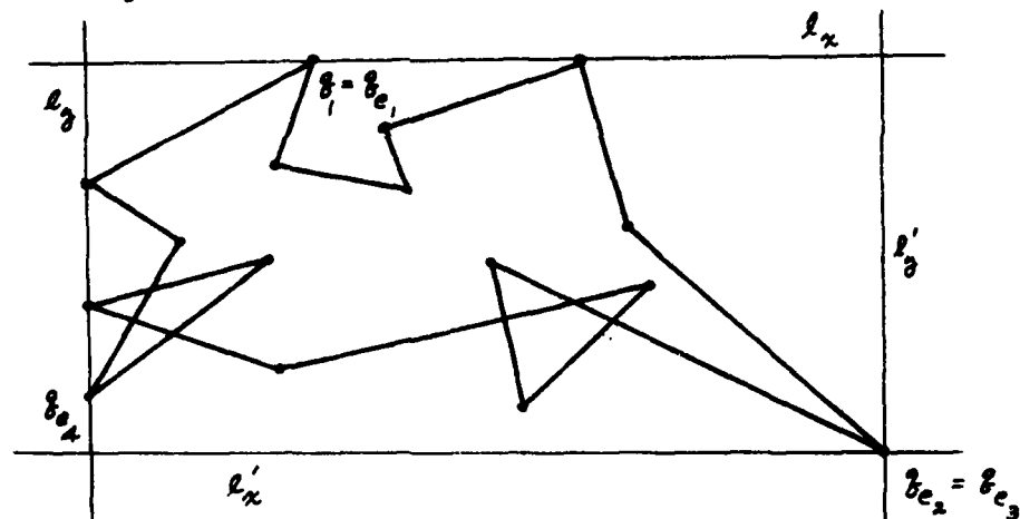
Figure 2. A polygon Q and its extreme points.
