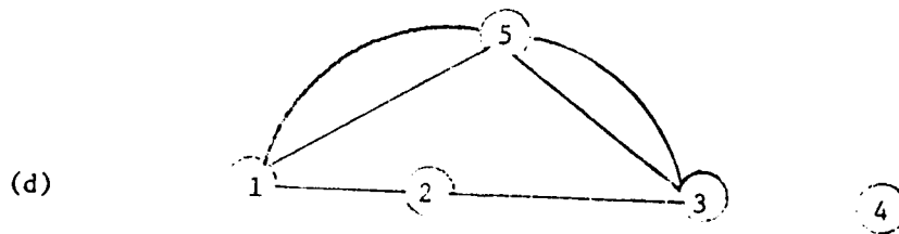
Figure 1. Examples of 2-trees on 5 Nodes
