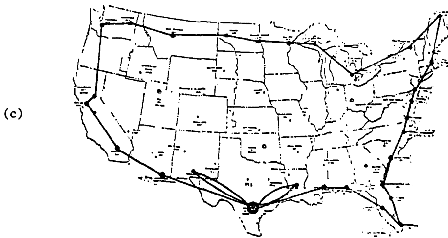
Figure 5. Illustration of Solutions to Problems On Network II.
