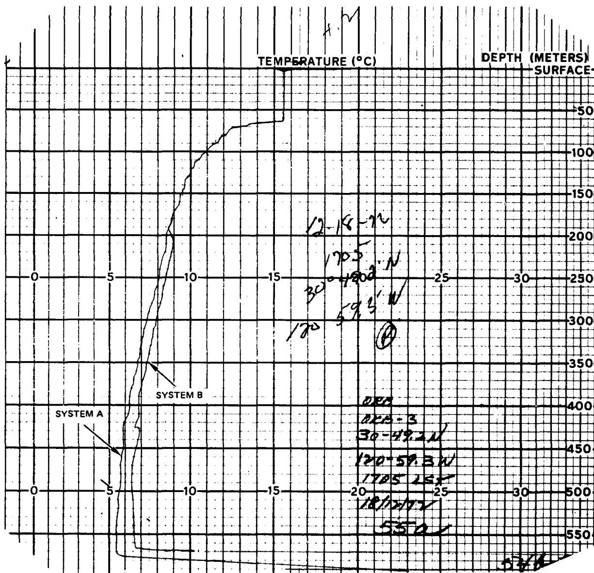
Figure 44b. Temperature profiles for ORB-3 XBT pair 54.
