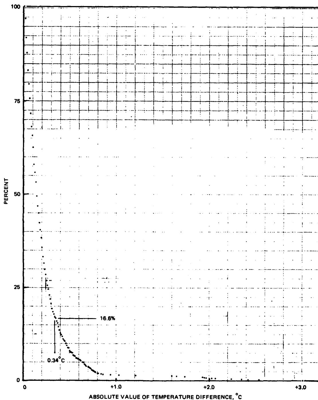
Figure 42. Ogive of the absolute value of 1116 simultaneous XBT temperature differences measured at standard hydrocast depths from the surface to 400 meters during the ORB-3 and RAPLOC/DEEPTOW experiments.
