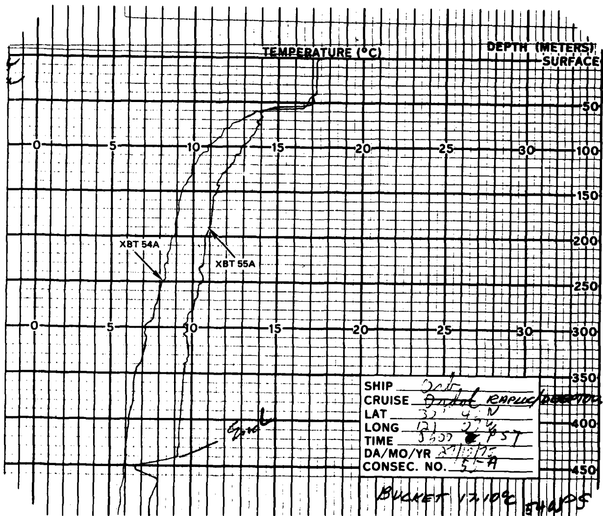
Figure 37. RAPLOC/DEEPTOW XBT profiles 54A and 55A.
