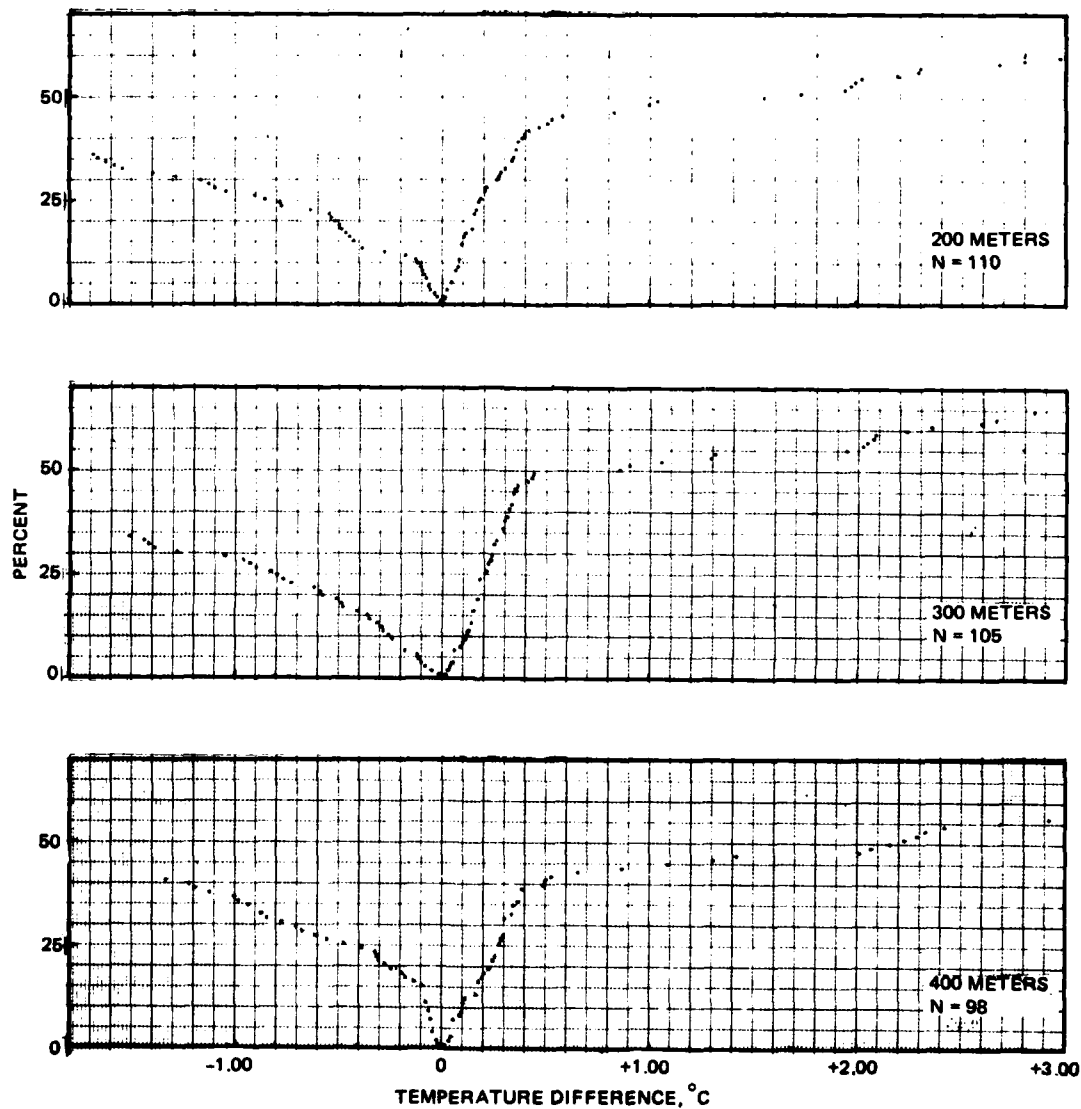
Figure B-3. Positive and negative ogives of CAPER water mass 2 temperature differences between average hydrocast and STD/SV and XBT profile measurements.
