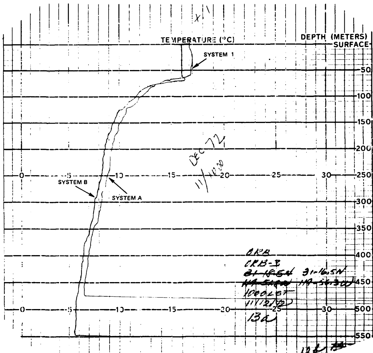
Figure 43b. Temperature profiles for ORB-3 XBT pair 12.
