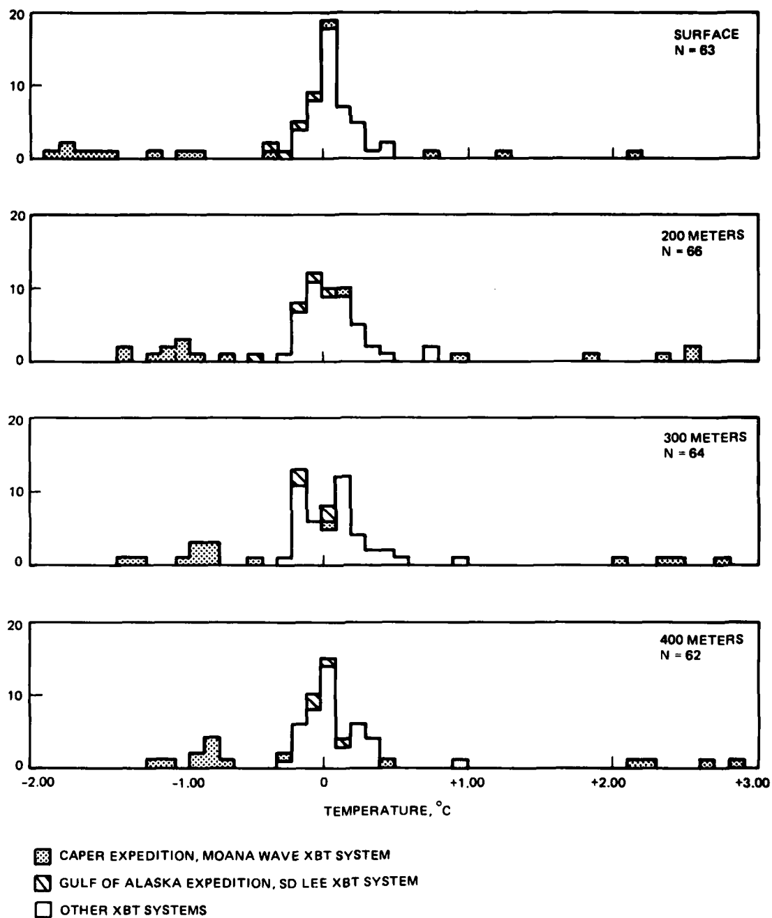
Figure 27. Differences between quasisimultaneous XBT and STD/SV temperatures.
