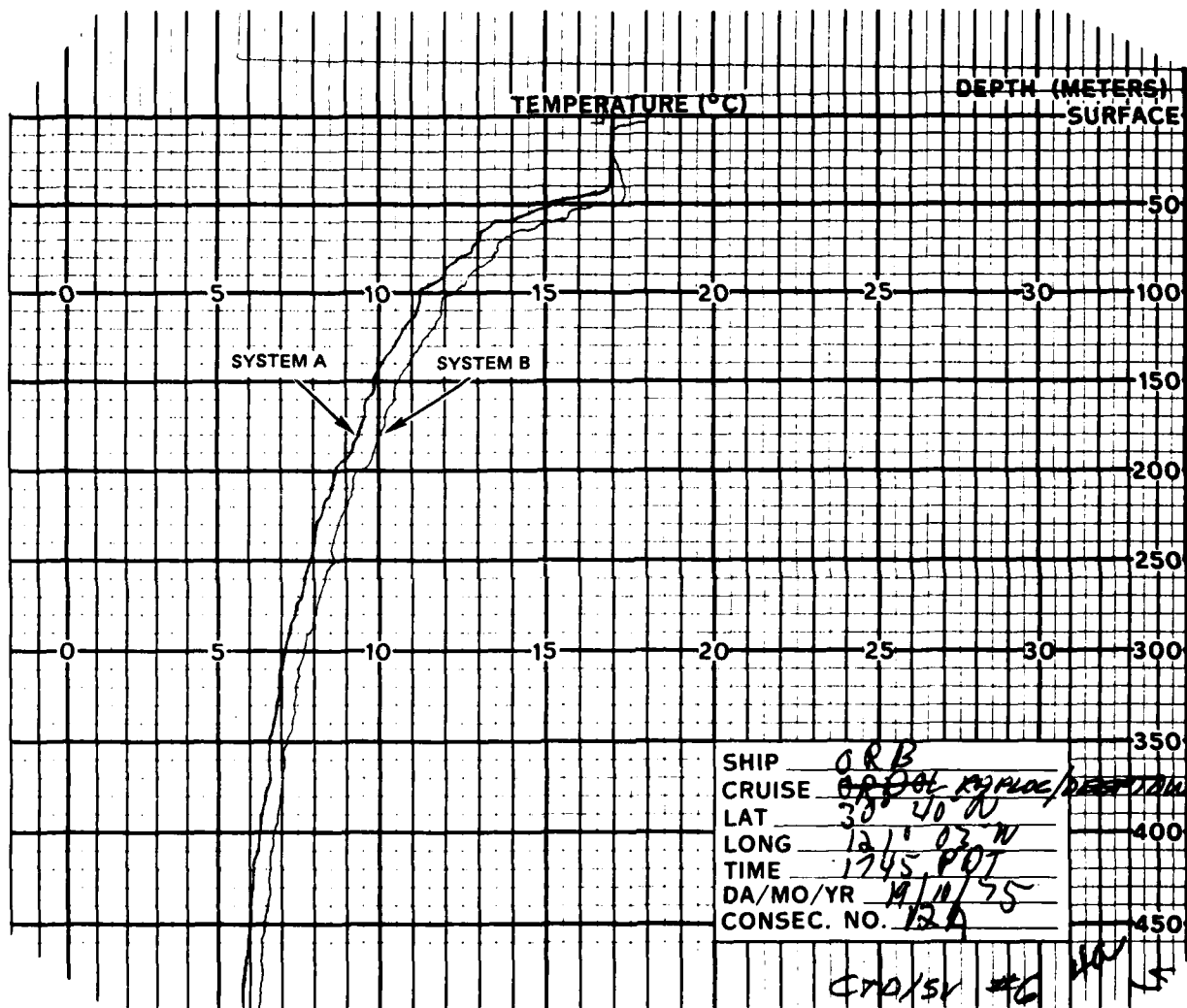
Figure 46a. Temperature profiles for RAPLOC/DEEPTOW XBT pair 4.
