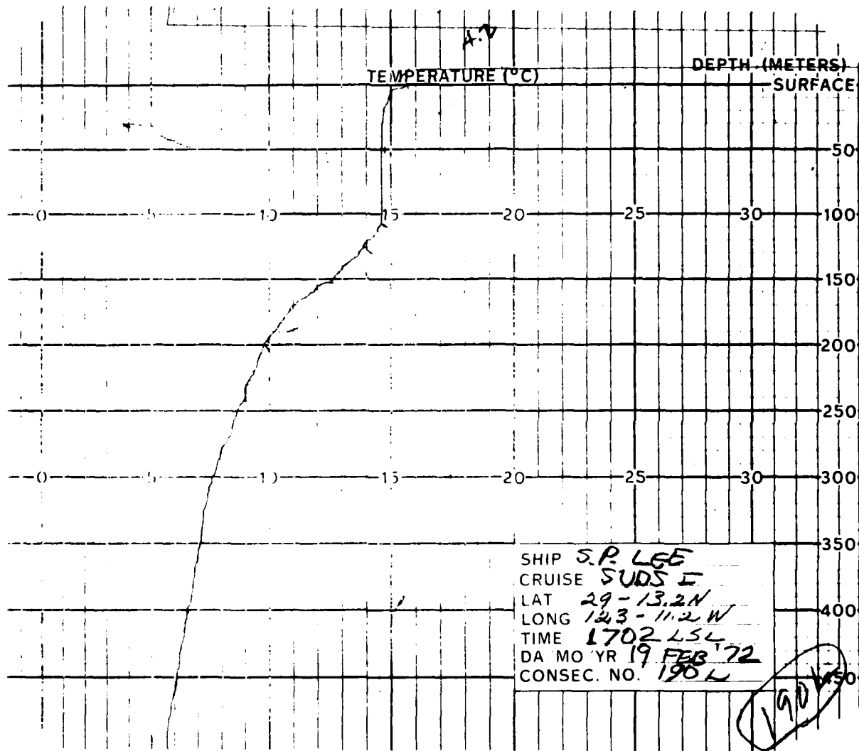
Figure 14a. SUDS I XBT 190L.
