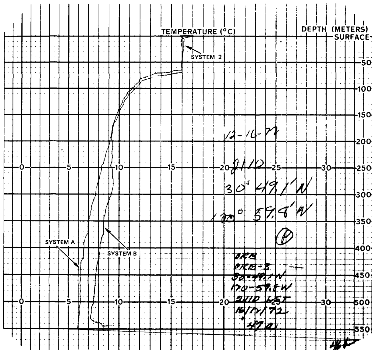
Figure 44a. Temperature profiles for ORB-3 XBT pair 46.
