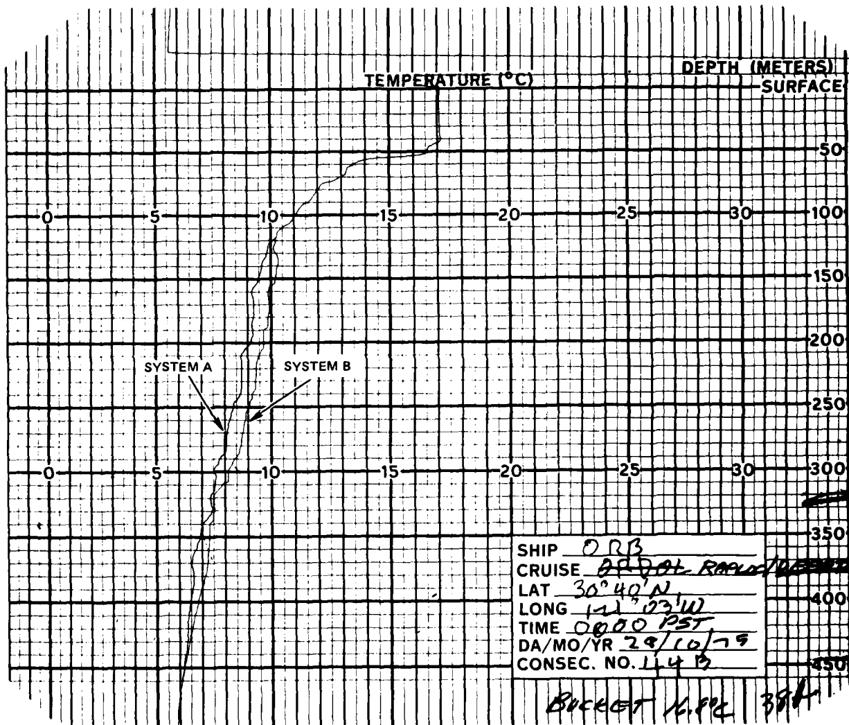
Figure 45b. Temperature profiles for RAPLOC/DEEPTOW XBT pair 38.
