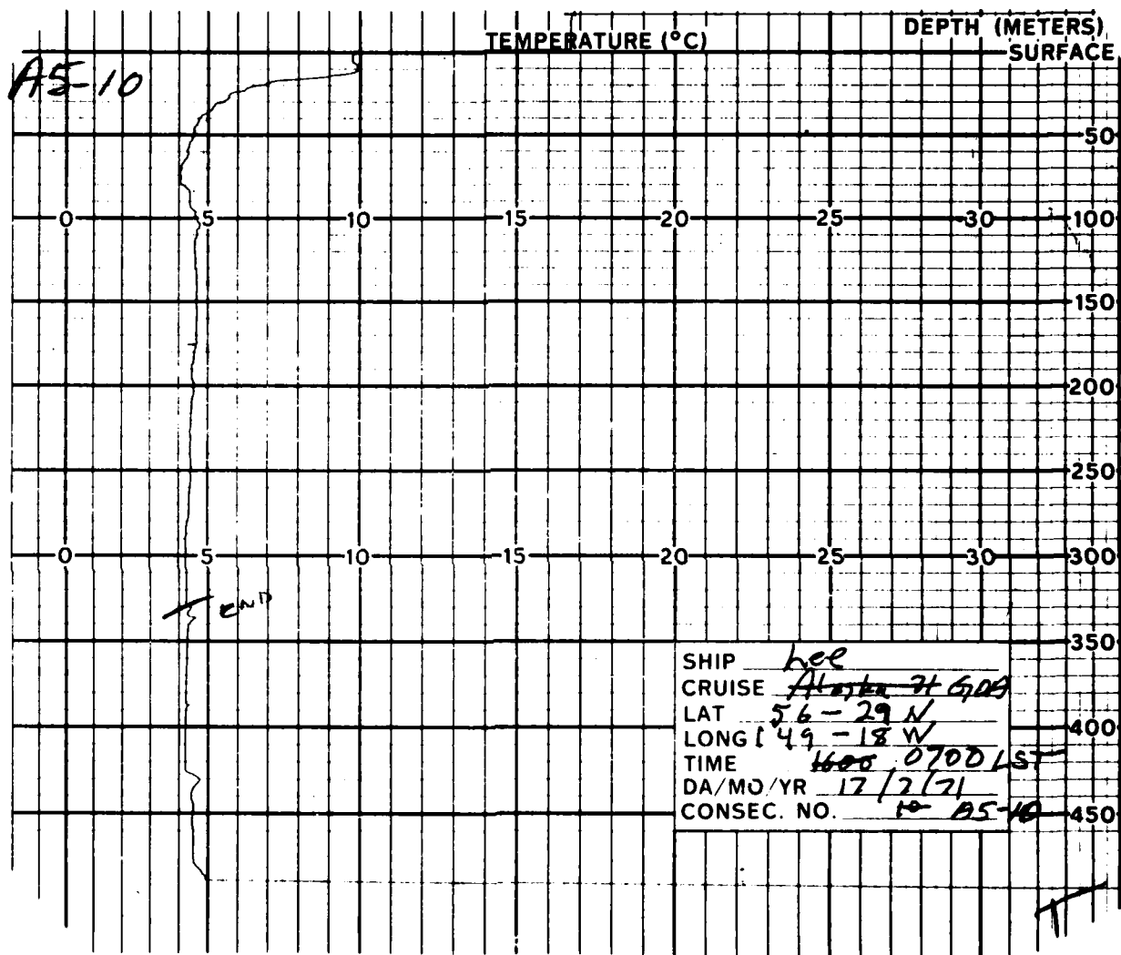
Figure 18. Gulf of Alaska XBT 302.
