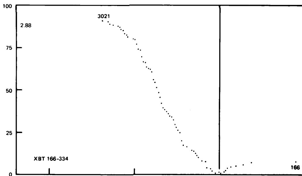
Figure 16. Ogives of positive and negative differences between Gulf of Alaska XBT surface temperatures and towed thermistor temperatures.
