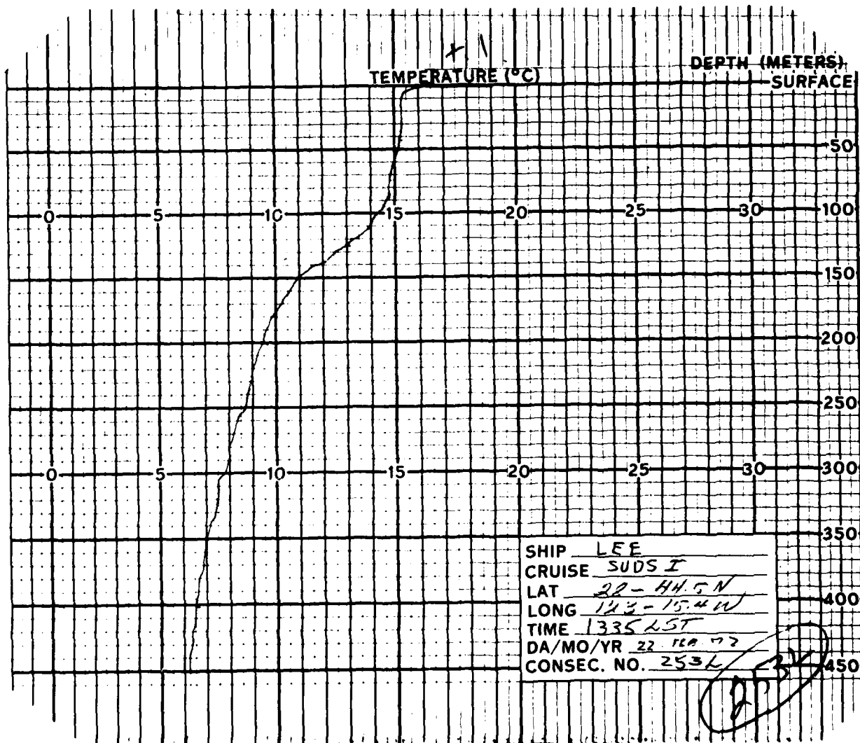
Figure 14b. SUDS I XBT 253L.
