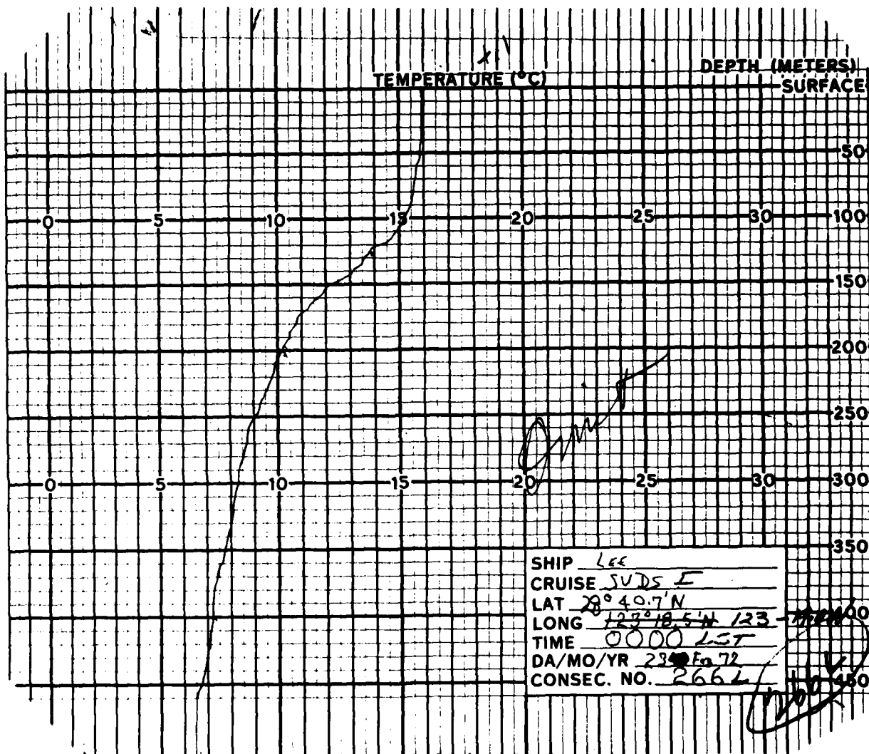
Figure 34. SUDS I XBT profile 266L.
