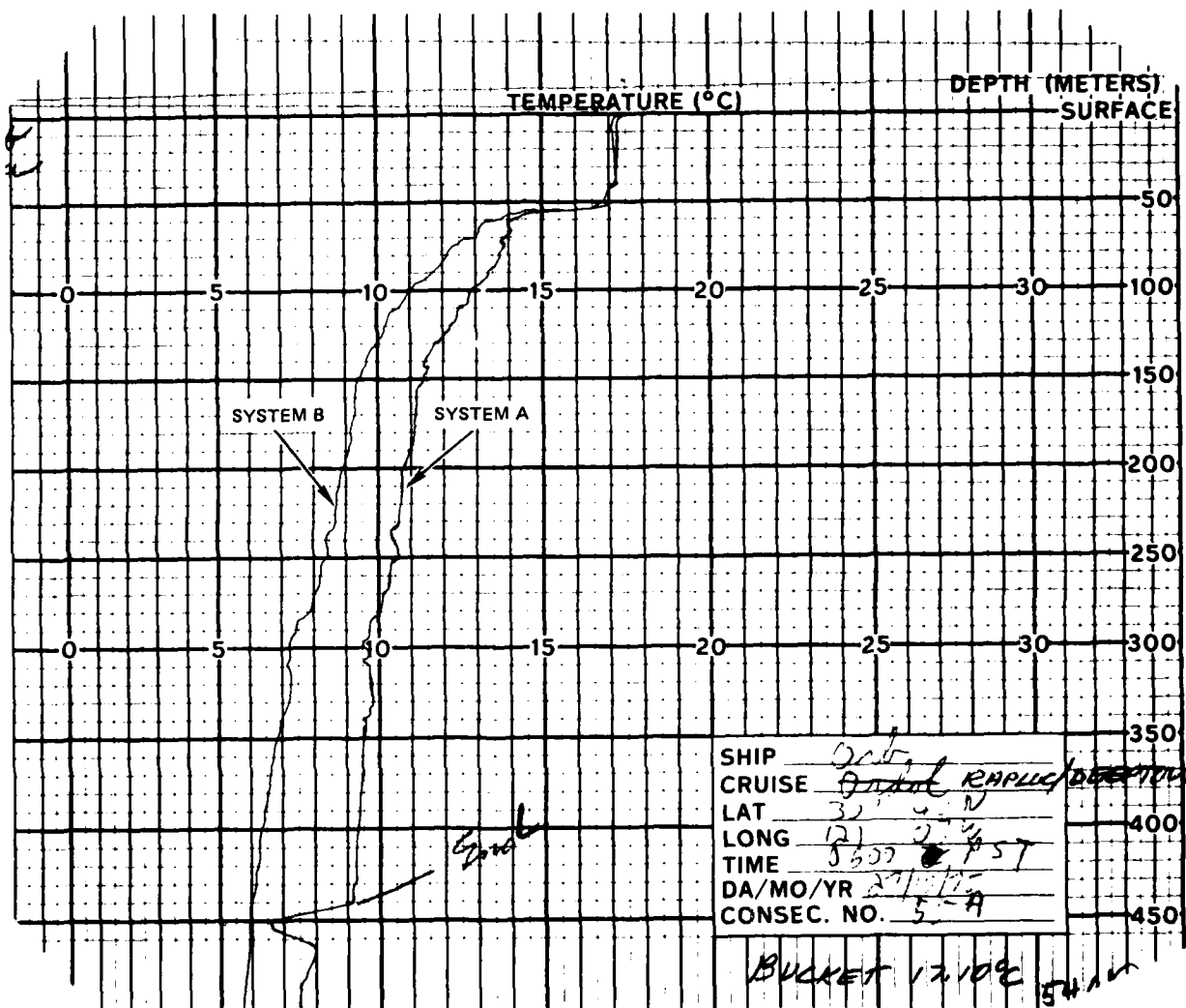
Figure 45a. Temperature profiles for RAPLOC/DEEPTOW XBT pair 33.
