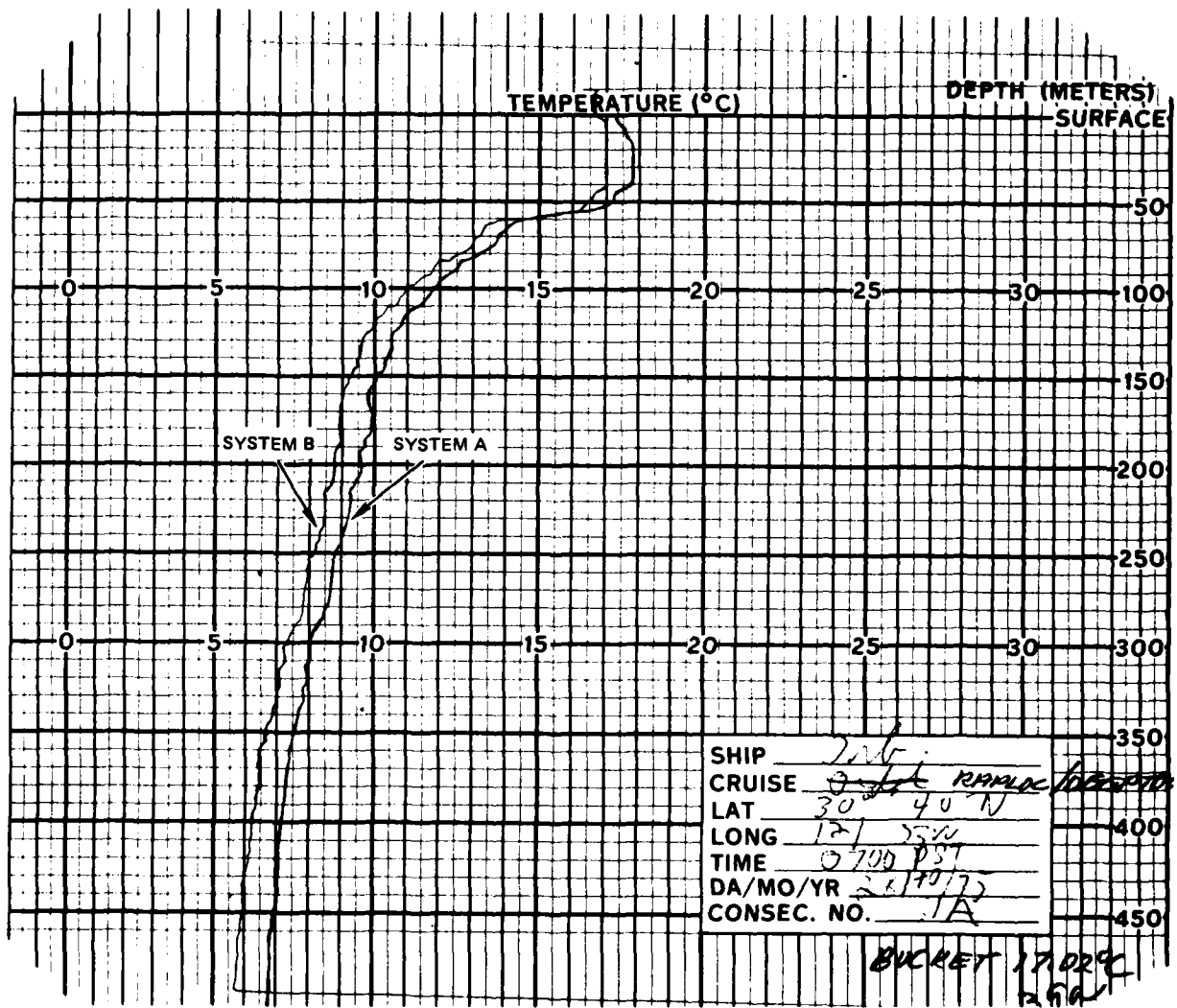
Figure 46b. Temperature profiles for RAPLOC/DEEPTOW XBT pair 39.
