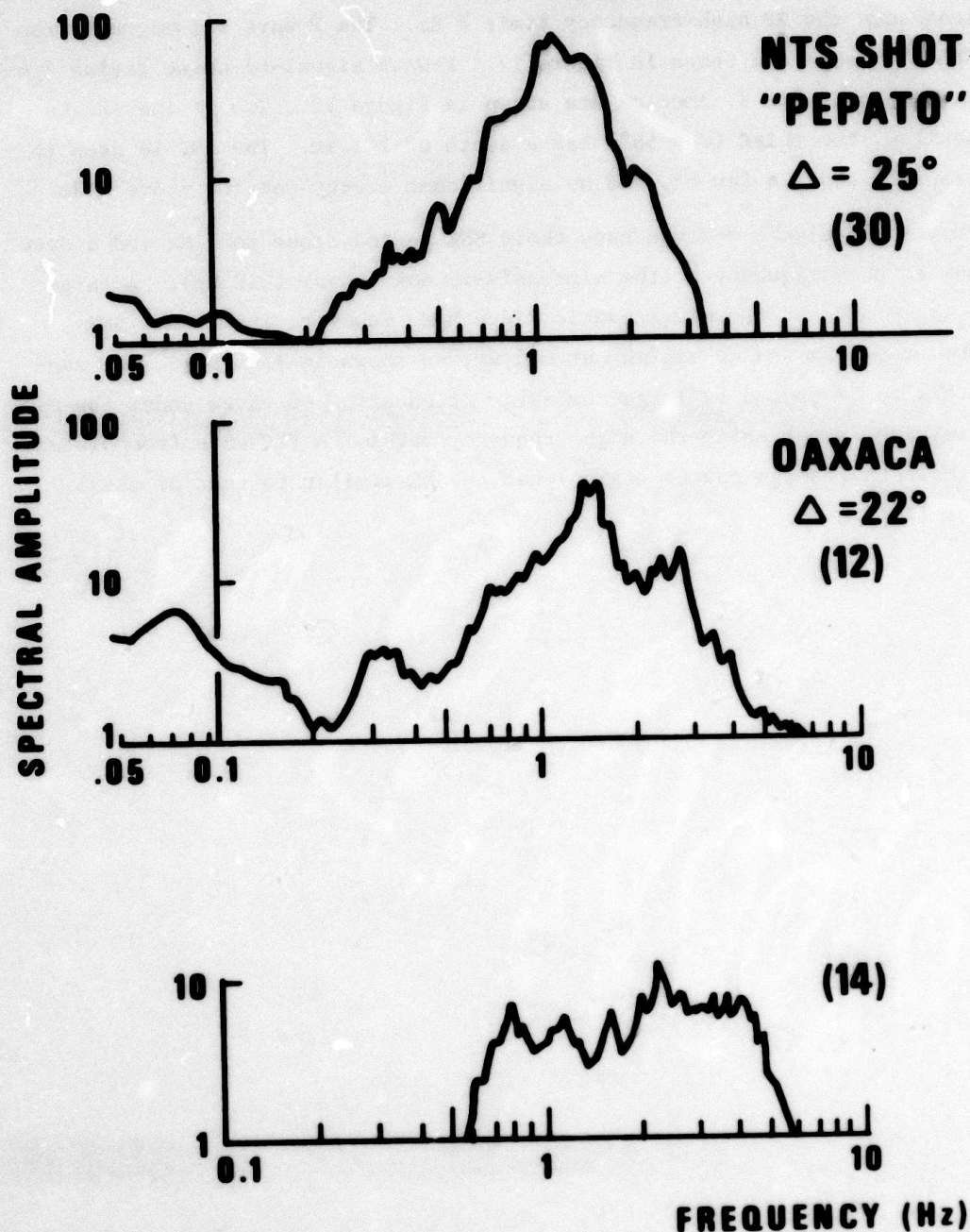
Figure 16. Signal-to-noise ratios of P-waves, measured by spectral amplitude ratio, of an NTS shot and of two earthquakes in Oaxaca, Mexico. Numbers in parentheses refer to event list in App. 1.
