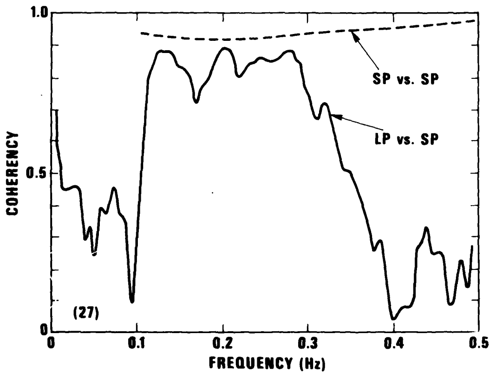
Figure 12. Coherencies computed between the NSS MP (top figure) and LP (bottom figure) traces against the SDCS SP traces, compared to the NSS SP vs SDCS SP coherency (broken lines). The coherencies are high up to 60% of the folding frequency of the respective MP or LP instrument.
