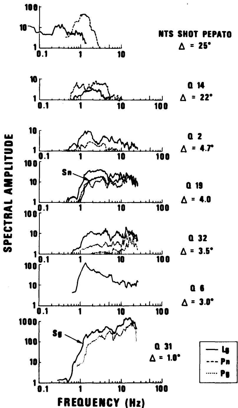
Figure 14. Signal-to-noise ratios (measured by spectral amplitude ratio) of regional seismic phases from events in the distance range 1° to and 22° to 25°. Quake numbers refer to App. 1.
