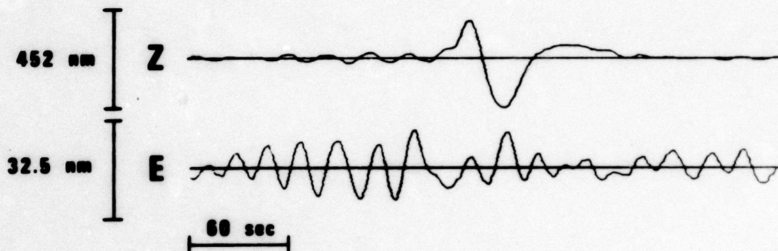
Figure 8. NSS MP (top) and LP (bottom) recordings of an earthquake ( \Delta = 1.0^\circ , m_s(LG) = 3.6^\circ ) showing a spurious-looking long-period oscillation on the vertical channels. We suggest this to be a non-linear response to the large high-frequency earth motion. Vertical channel is marked by Z, east-west component by E. No north-south channel was recorded.
