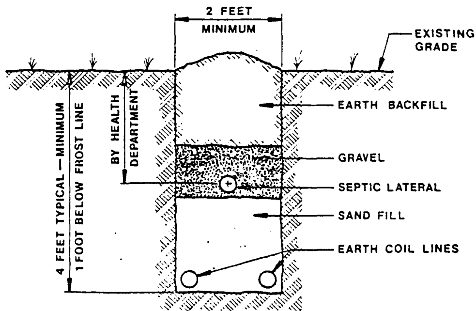
Figure 12 Earth Coil Plan and Cross Section [Partin, 1980, 2]
