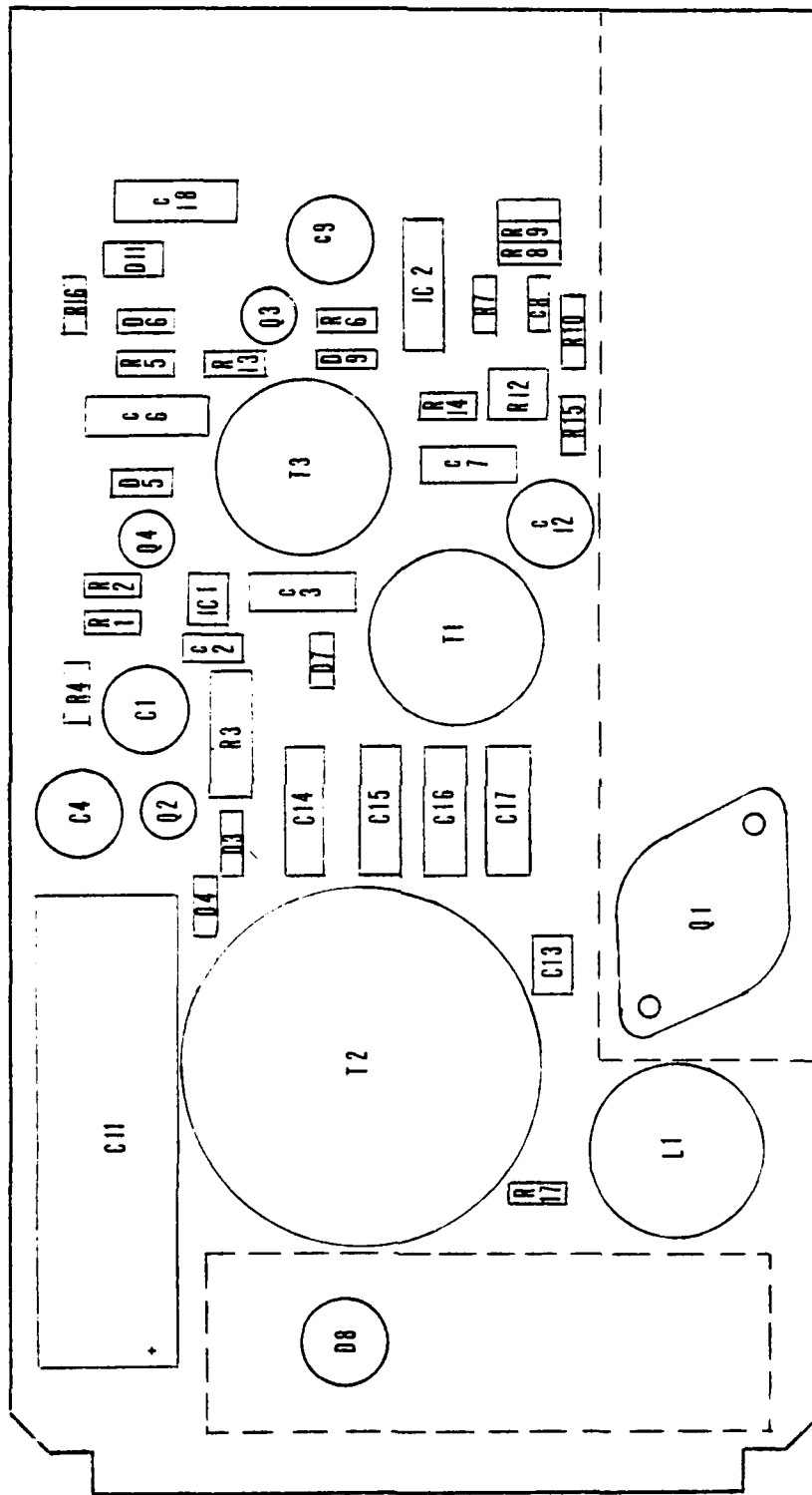
5 V, 35 W DC to DC Converter Component Layout
