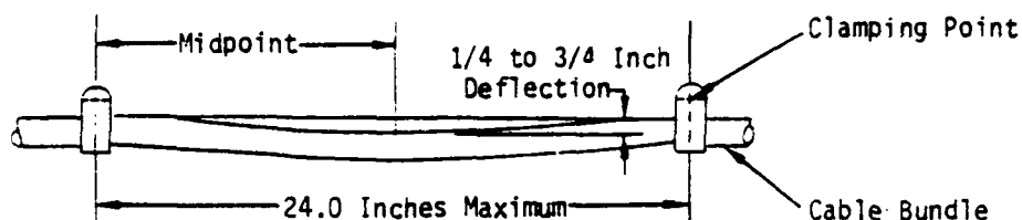
FIGURE 1. SLACK IN CABLING
