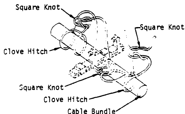
DETAIL METHOD OF SECURING BUNDLES TO SUPPORTS
