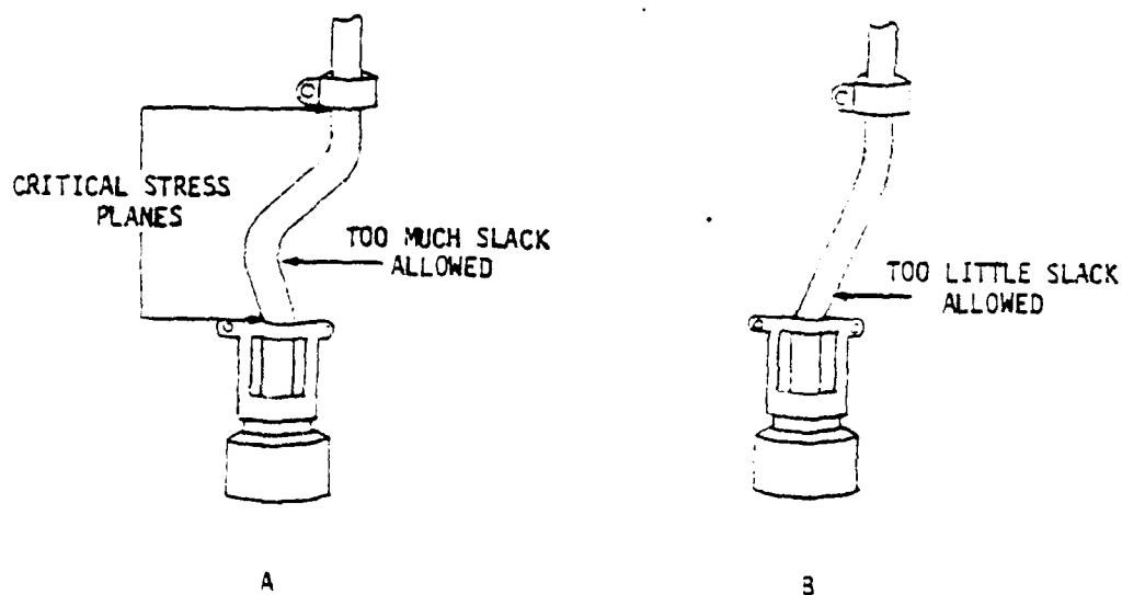
ILLUSTRATION 2: UNACCEPTABLE INSTALLATION
