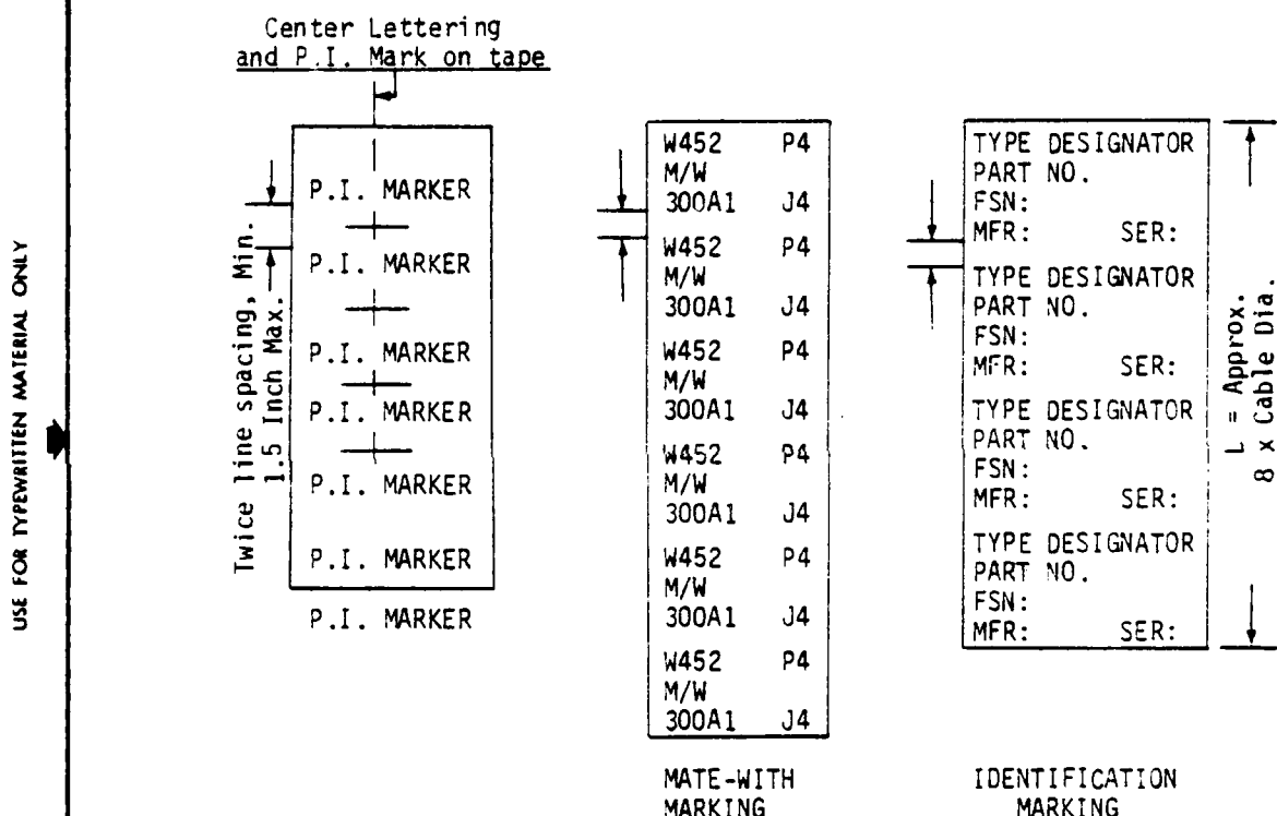
FIGURE 2. TAPE MARKING BAND, REPETITIVELY PRINTED
