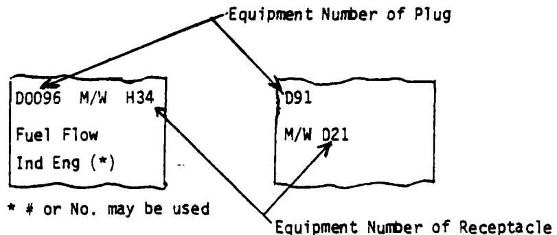
FIGURE 1. EXAMPLES OF MATE-WITH MARKERS
