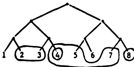
Figure 5.1 A cone graph with 4 hyperedges
