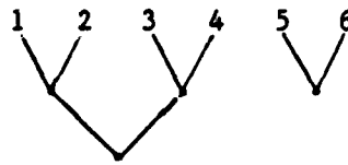
Figure 4.1 A 2SSG of S_6 .
