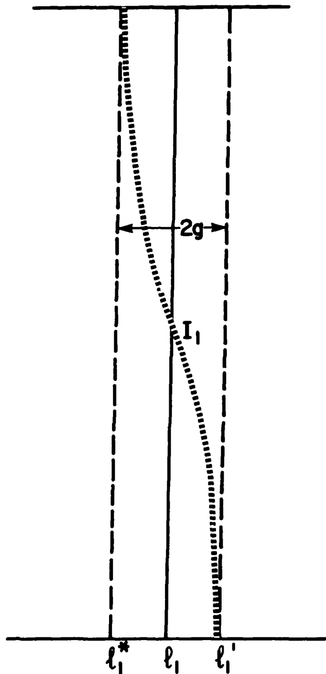
FIG. 20(b) SCHEMATIC DRAWING OF THE CURVED SHOCK IMAGE I_1 AT LEFT, SHOWING THE LINES l_1^* AND l_1' WHICH ARE PARALLEL TO w_v (THE Y-DIRECTION), THE SHOCK POSITION l_1 MIDWAY BETWEEN THEM, AND THE AMPLITUDE g OF THE DISTURBED SHOCK FRONT, EXAGGERATED HERE FOR THE PURPOSE OF ILLUSTRATION. IN (a) 2g = 3.7 mm. I_1 CONSISTS OF THE BASIC GEOMETRIC UNIT, THE COSINE HALF-WAVE, WHICH IS PERPENDICULAR TO THE TOP AND BOTTOM WALLS. NOTE THAT I_1 CROSSES l_1 JUST ONCE.
