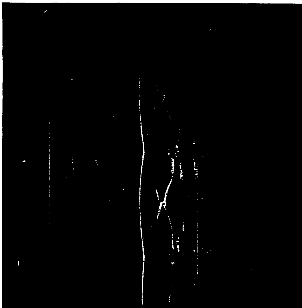
FIG. 10 (a) MULTIPLE-EXPOSURE SCHLIEREN PICTURE OF AN IONIZING SHOCK WAVE MOVING LEFT IN AIR. M_0 = 10.1 , P_1 = 0.79 TORR, T_1 = 293.15 K, t_p = 0.0001 (RUM NO. 1).
