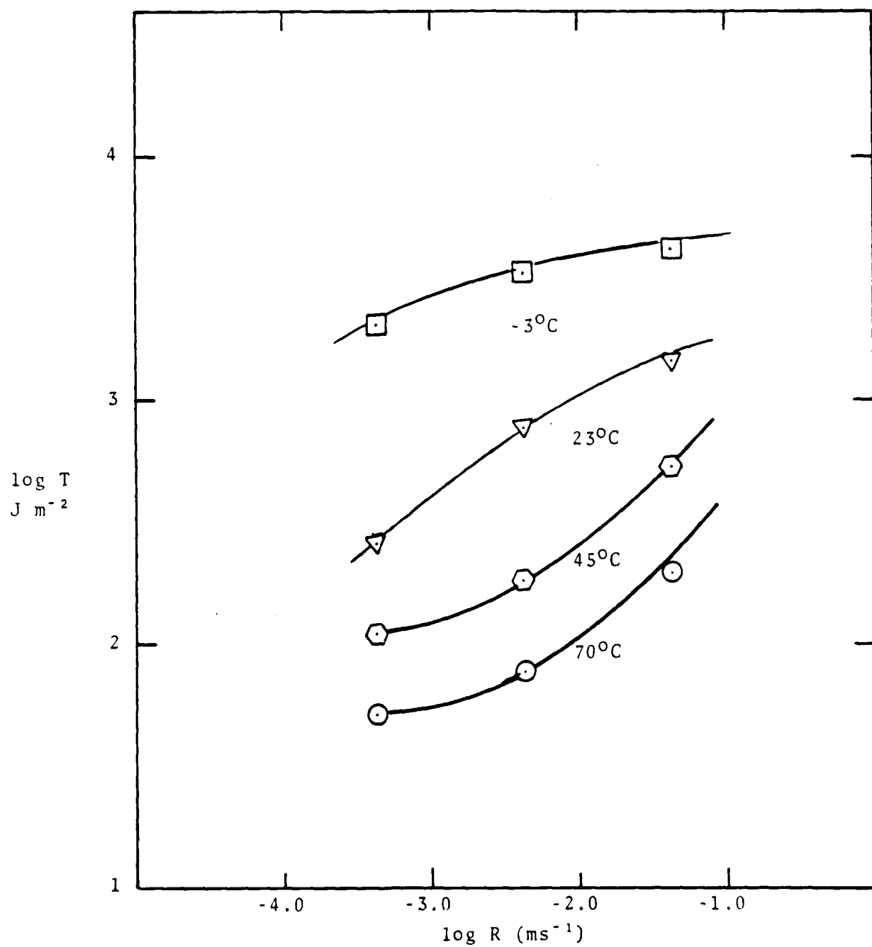
Figure 17. Temperature and rate effects on tearing energy T for sample TB 11 .
