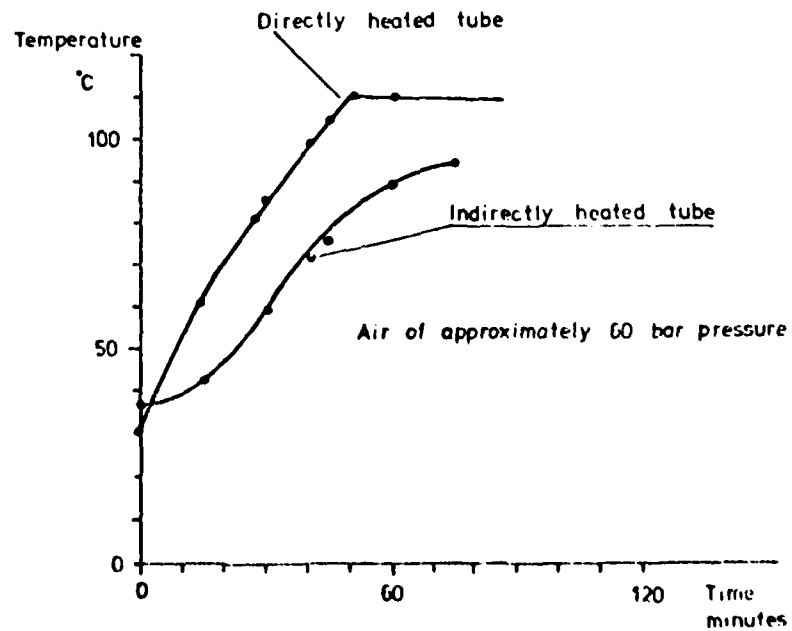
Figure 3. Wall temperatures in the heated tub array during a heating cycle.
