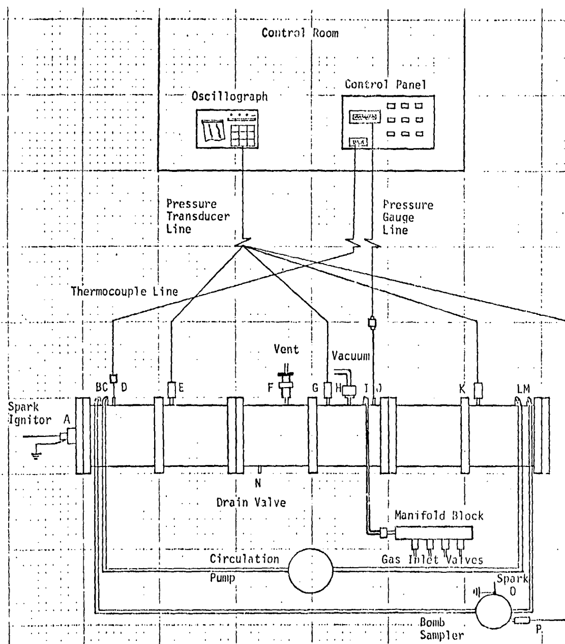
Figure B-2. Schematic Diagram of Flame Tube Test Equipment
