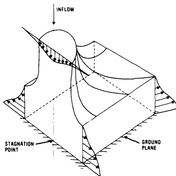
Figure 19. Jet impingement near ground level.
