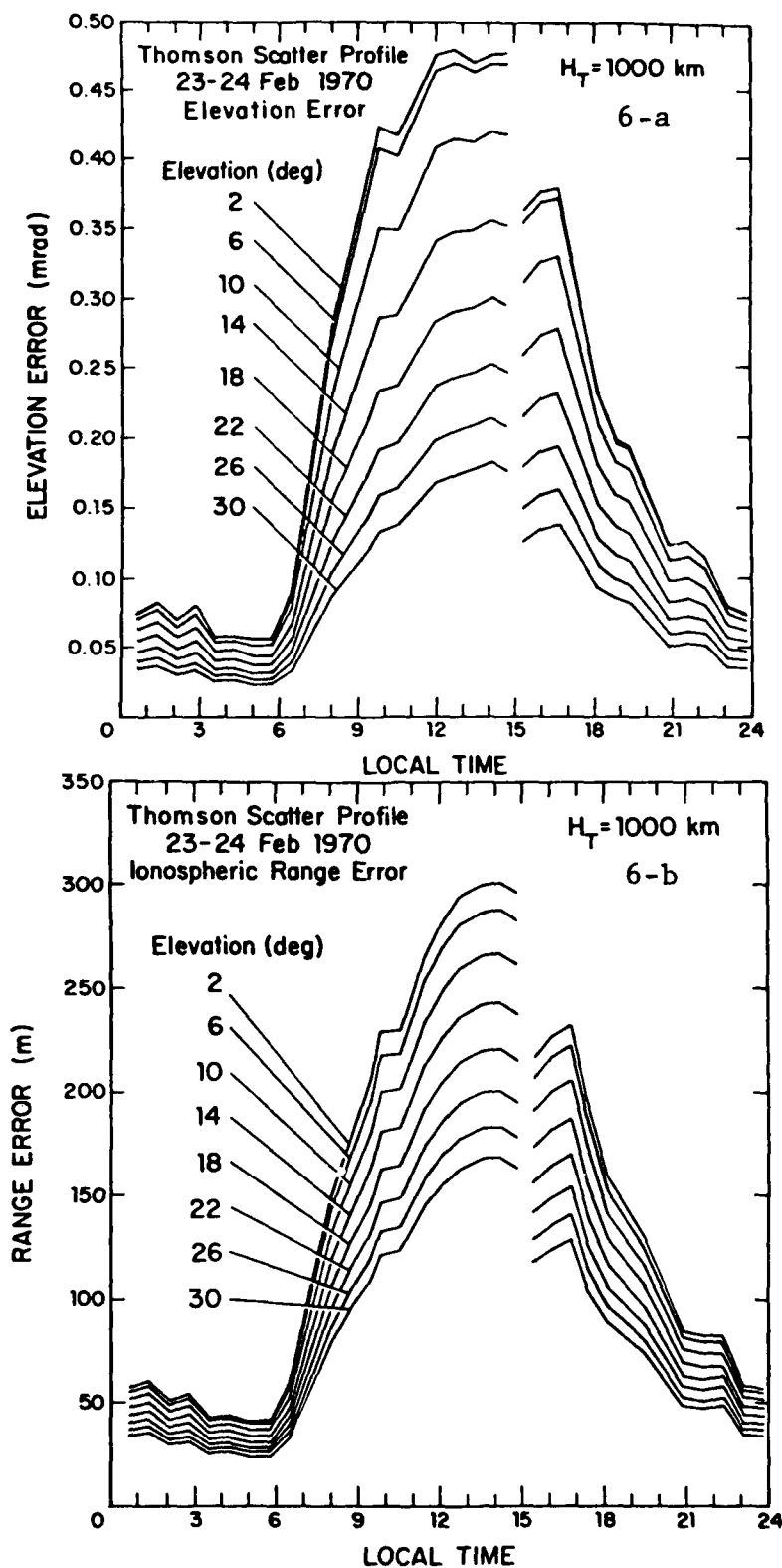
Fig. 6 — Ionospheric refraction (a) and range (b) errors at 400 MHz as deduced by ray tracing through Thomson scatter — derived electron density profiles. (From Evans and Wau [1975])
