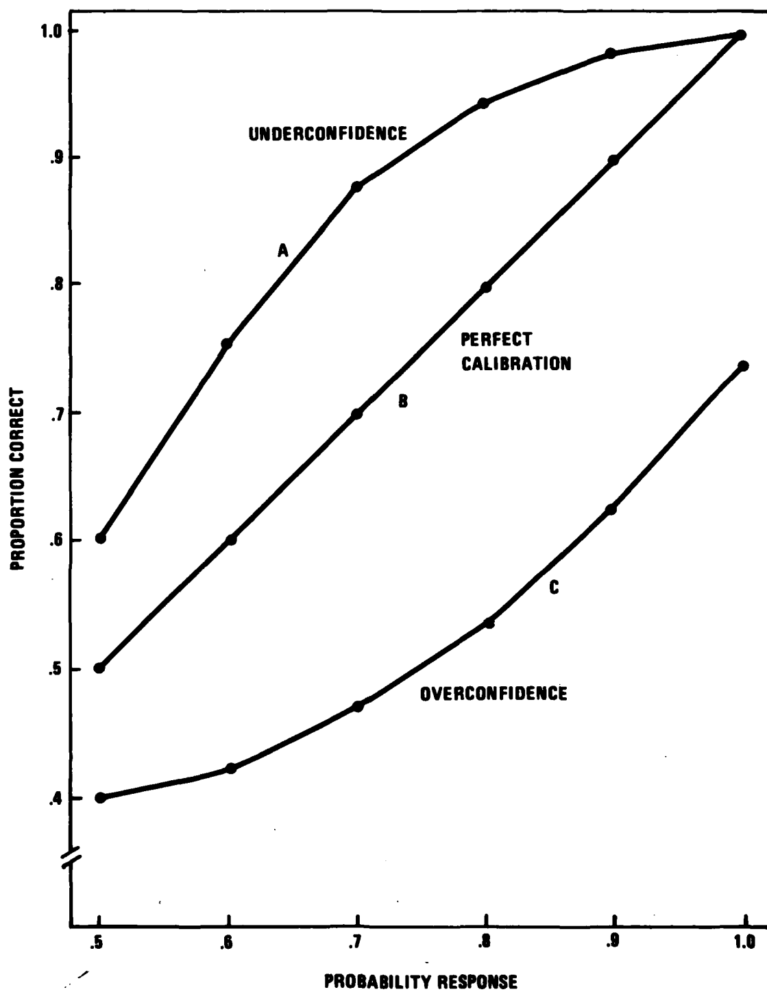
Figure 2. Idealized samples of perfect calibration, underconfidence, and overconfidence. Source. Lichtenstein and Fischhoff, 1978.
