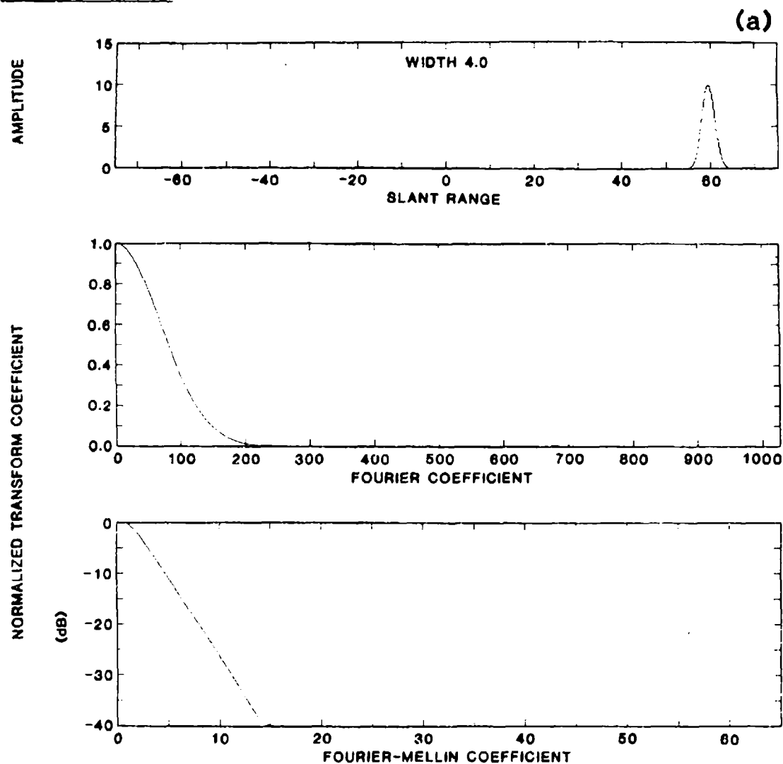
Fig. 5. Fourier and Fourier-Mellin transforms of sampled gaussian test functions illustrating the effects of shift and scale operations. Note also the effects produced by undersampling of the test function.
