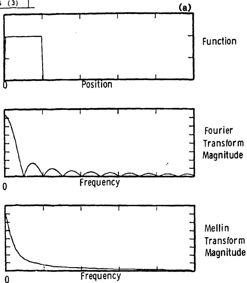
Fig. 3. Fourier and Mellin transforms of a rectangle test function illustrating how the magnitude of the Fourier transform is shift invariant while the magnitude of the Mellin transform is not. Similarly the Mellin transform magnitude is scale invariant while the Fourier transform magnitude is not.
