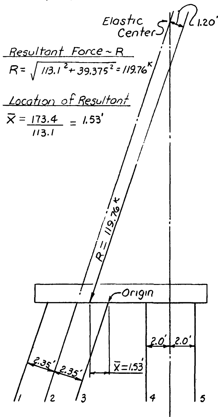
Force Diagram Forces resolved in direction of pile groups
