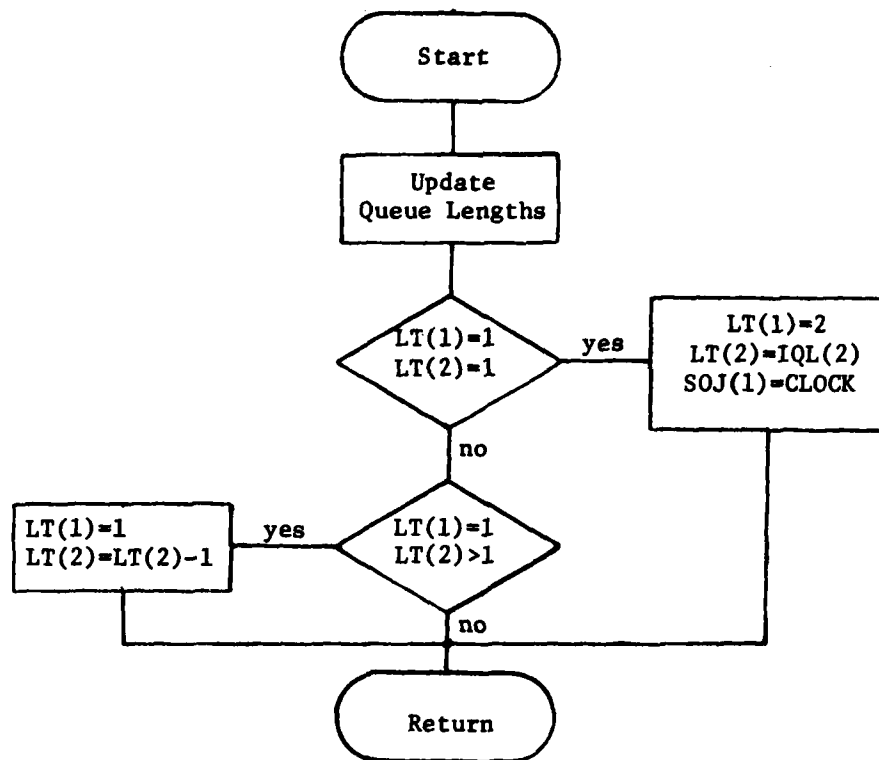
Subroutine DEPAB
