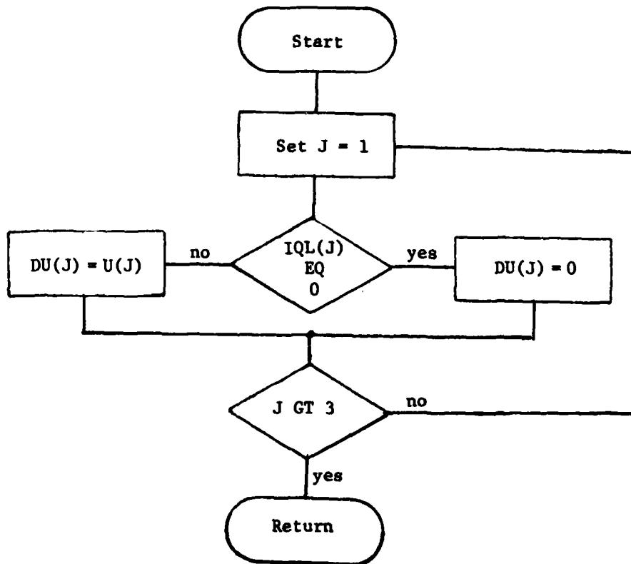
Subroutine CHECK
