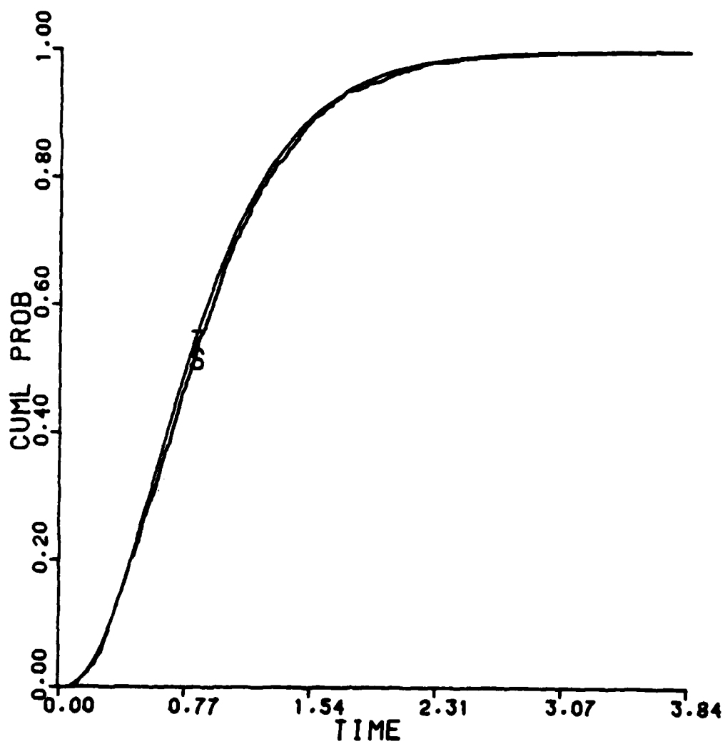
Figure 1.7. A Comparison Between a Sample Distribution, S, and one Assuming Independence, T
