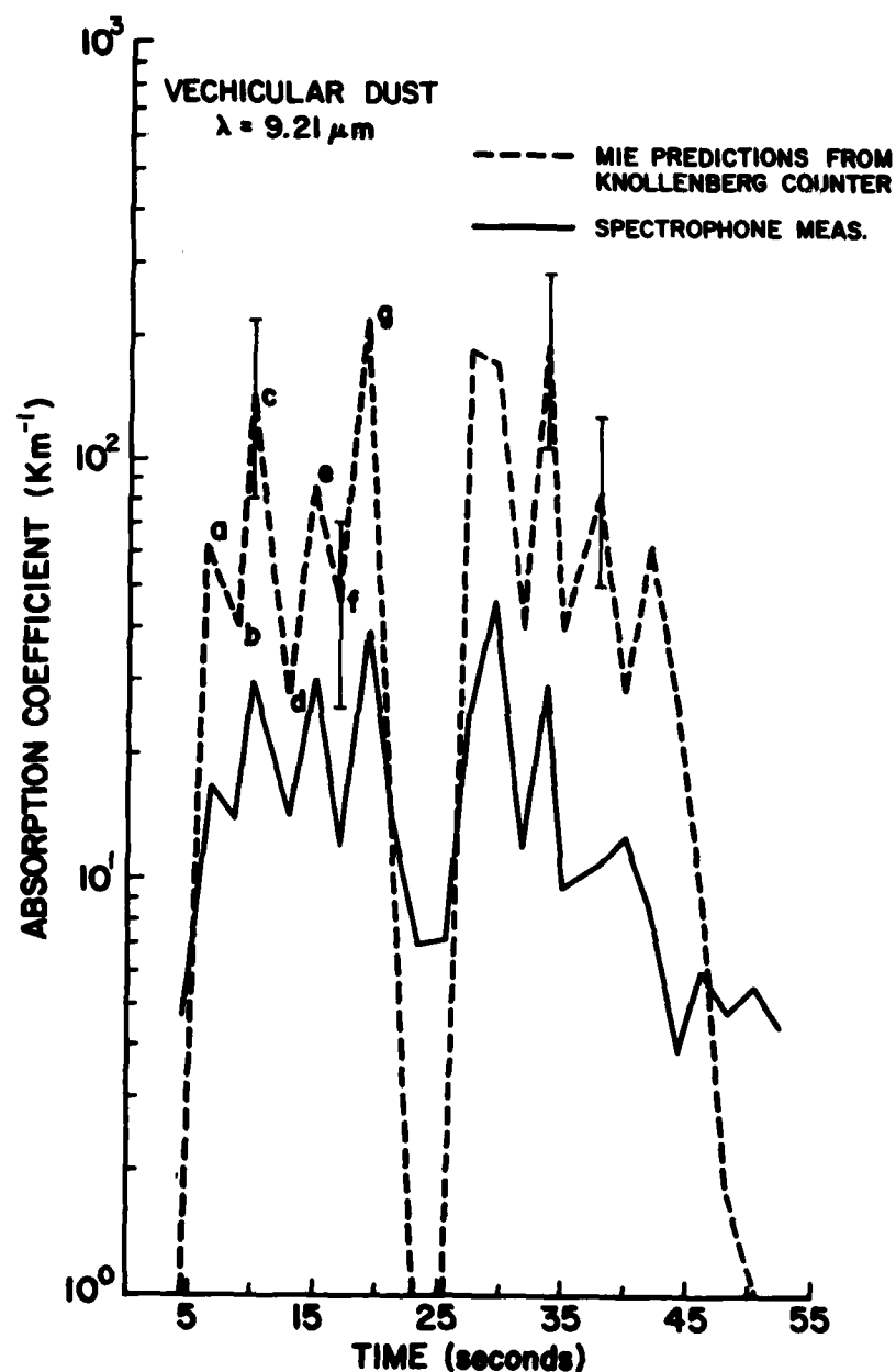
Figure 6. Absorption coefficient of vehicle dust at the 9.21 \mu\text{m} , R(34) \text{CO}_2 laser line as a function of time during the test: measured with in situ spectrophone (solid line); and calculated from particle size distribution measurements made with a Knollenberg light scattering aerosol counter (dashed line). The "error" bars superimposed on the Knollenberg-based predictions indicate only the error caused by uncertainty in particle size determination. Other sources of error in the predictions (see text) and differences in the spectrophone and Knollenberg probe sampling efficiencies are expected to cause the remaining discrepancy between measured and predicted absorption.
