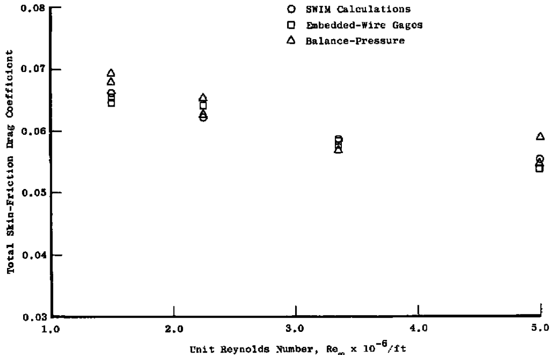
Figure 22. Total skin-friction drag coefficients at Mach number 0.6.
