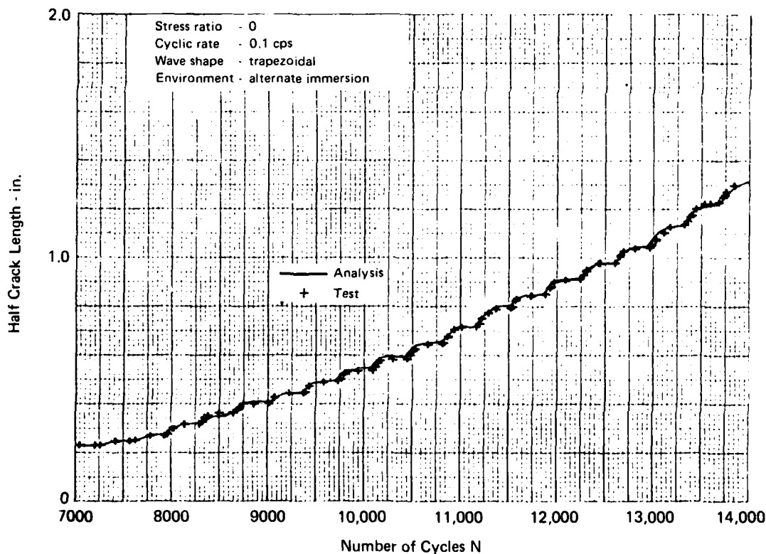
Figure 45. Crack Growth Behavior of 300M Steel in Alternate Immersion in Sea Water at Low Cycle Rates
