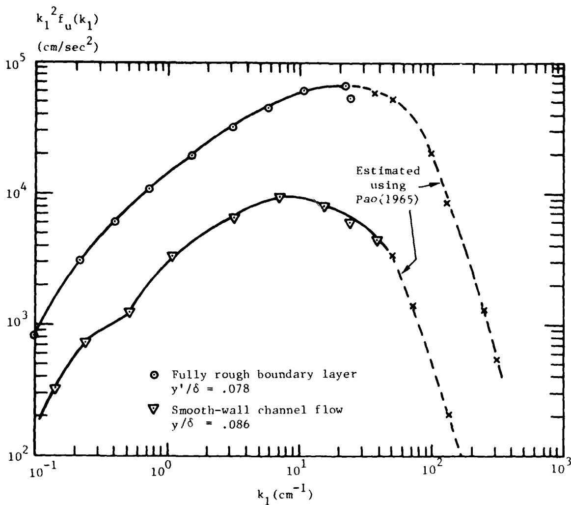
Fig. 3-30. Dissipation spectra in a fully rough turbulent boundary layer and a smooth-wall channel flow.
