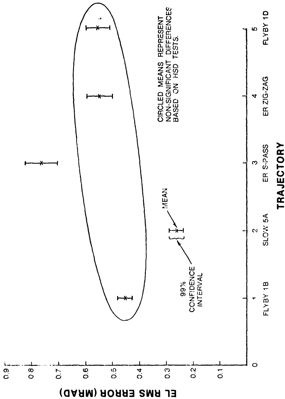
Figure 14. RMS Elevation Scatter Versus Trajectory with HSD Test Results
