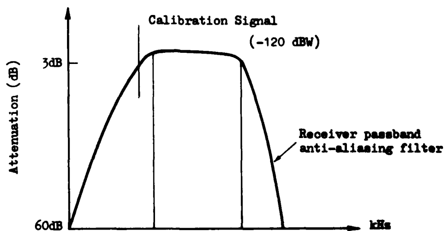
Figure 4. Sounder processing
