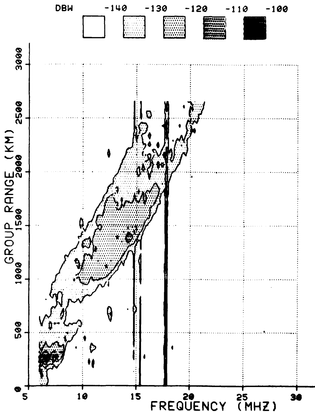
Figure 5. Backscatter ionogram
