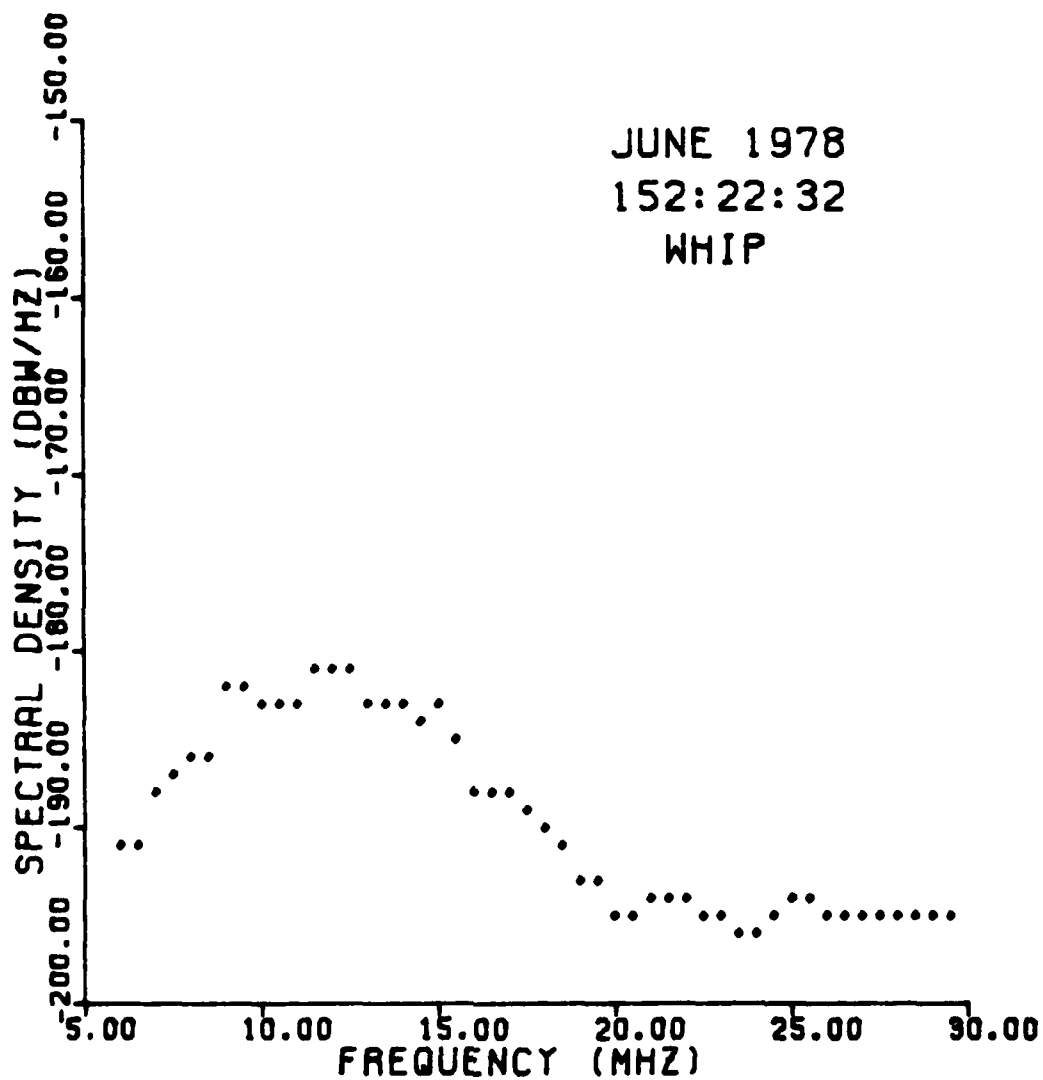
Figure 8. Atmospheric noise
